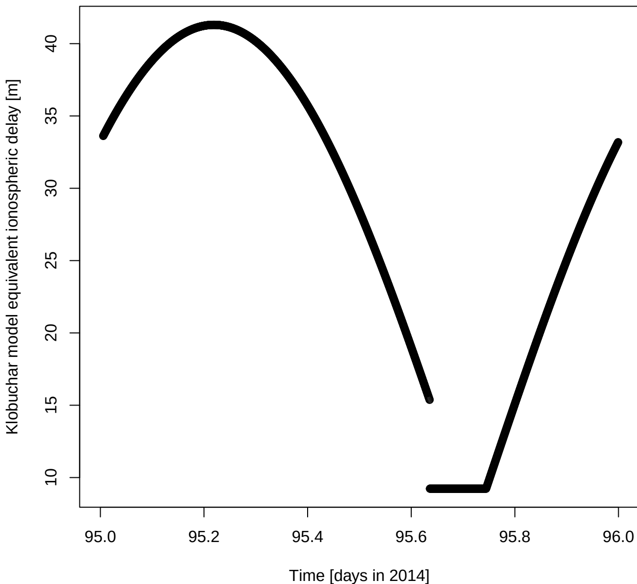
Klobuchar model equivalent ionospheric delay [m] for DOY 95 in 2014
