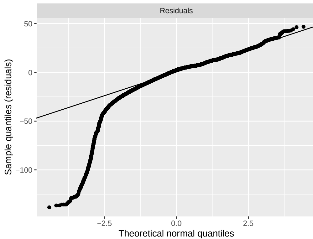
Q-Q plot for BCART residuals
