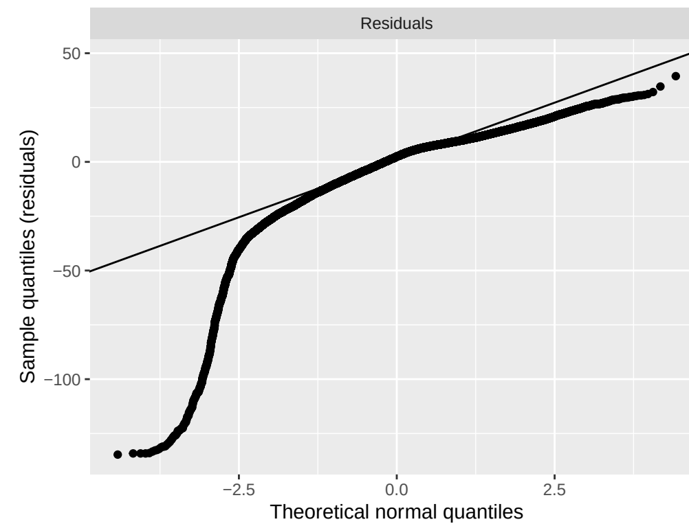
Q-Q plot for GAMB residuals
