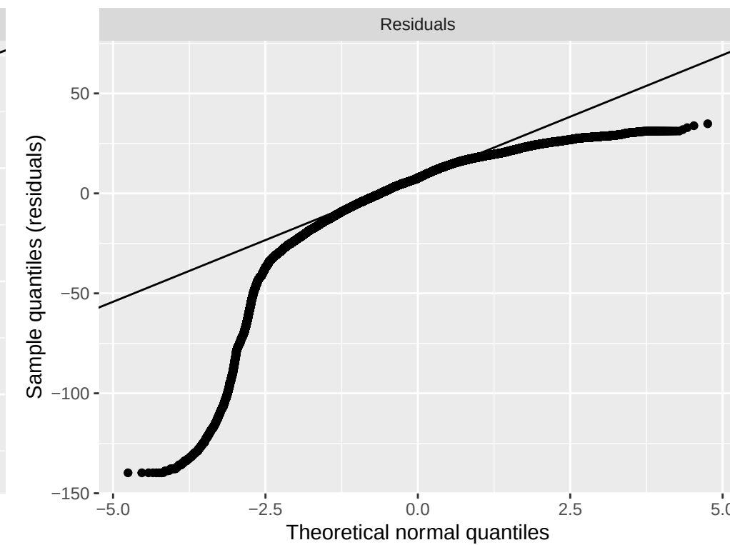
Q-Q plot for Klobuchar model residuals
