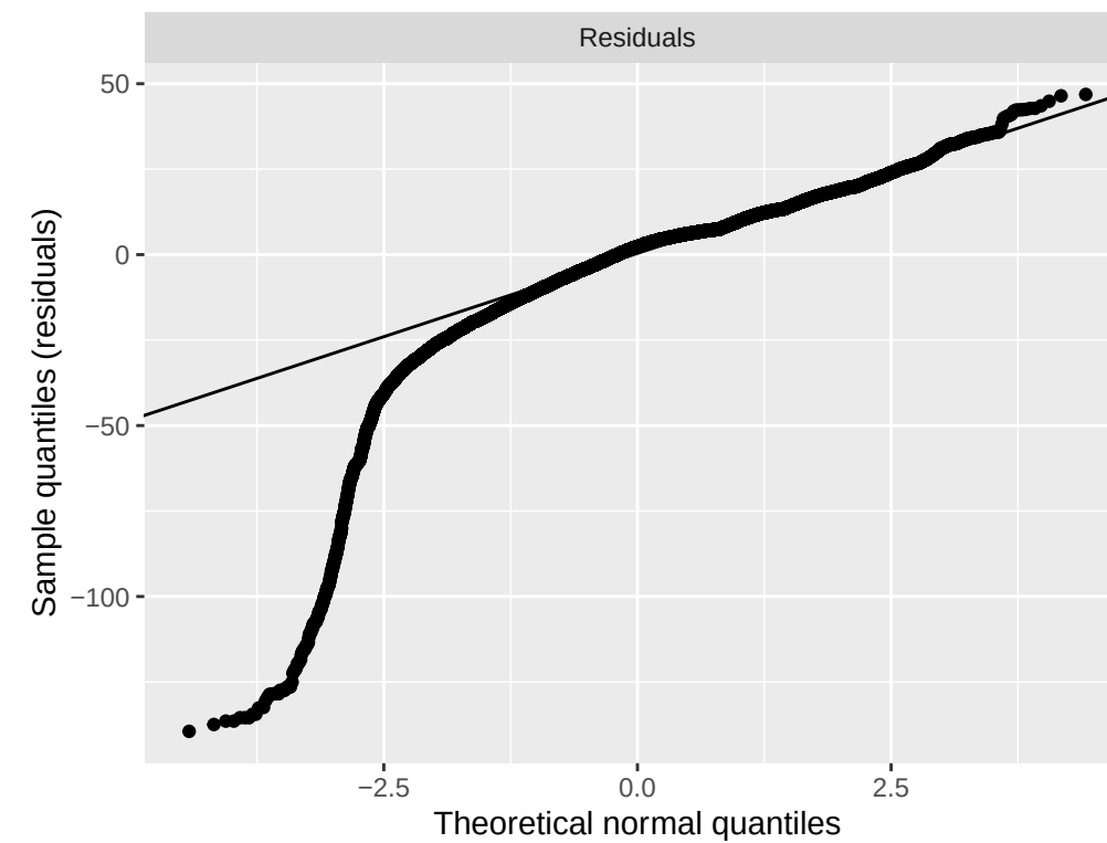
Q-Q plot for CART1 residuals
