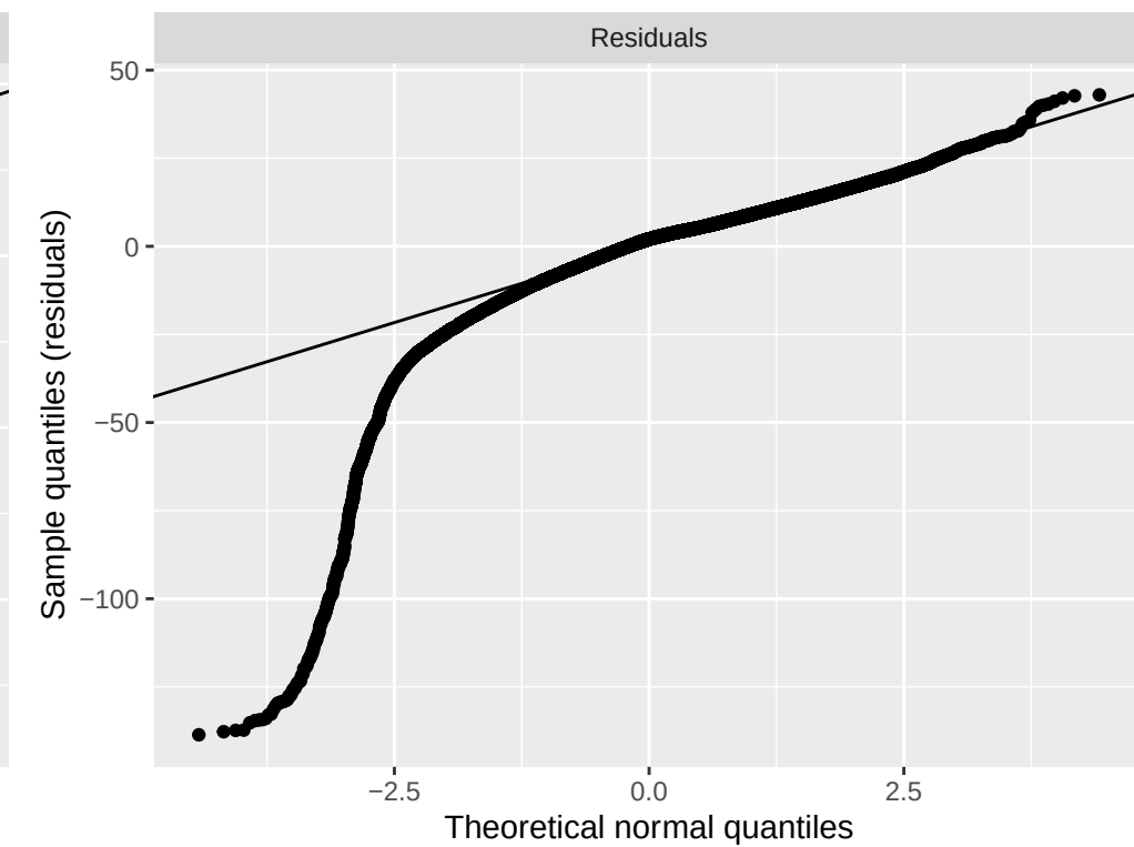
Q-Q plot for SGB residuals
