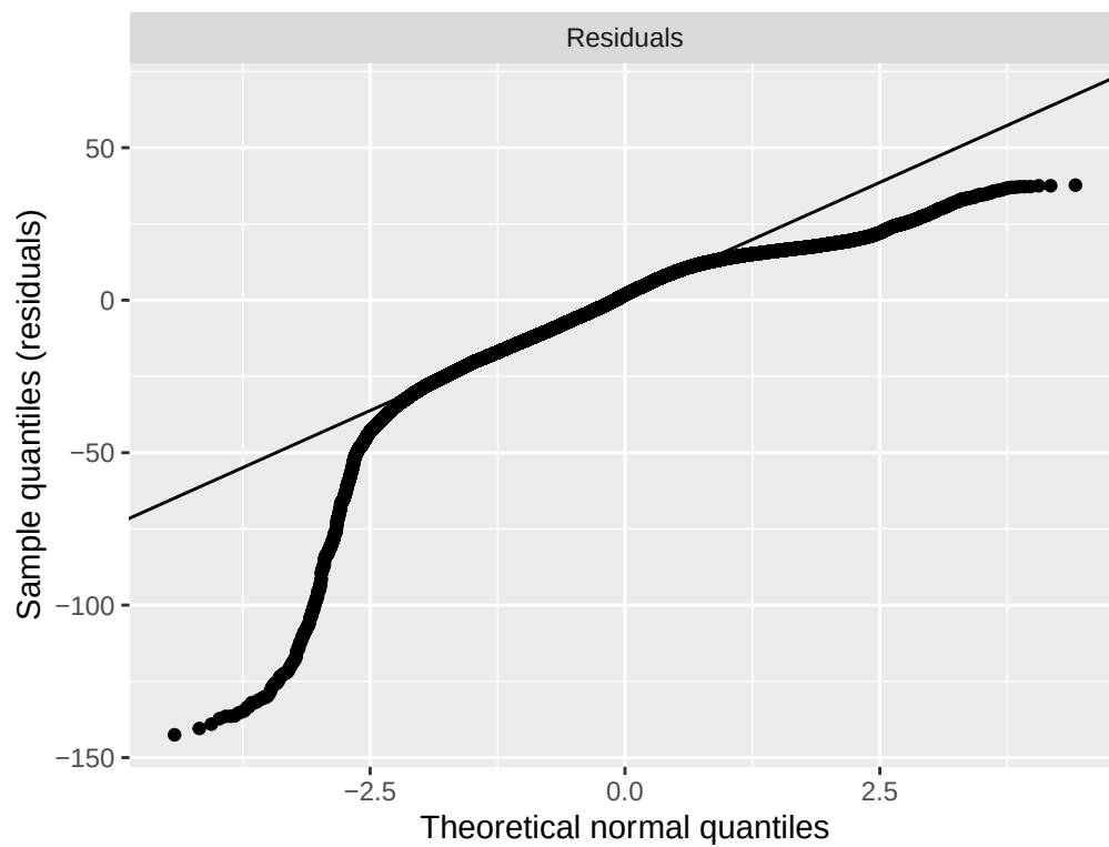
Q-Q plot for linear regression residuals
