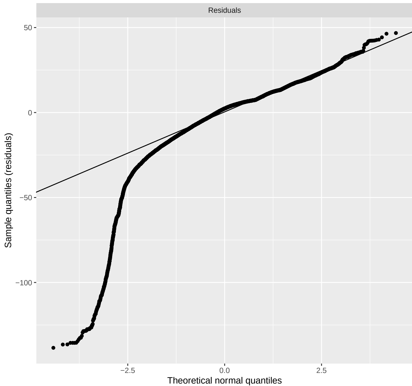
Q-Q plot for BCART residuals
