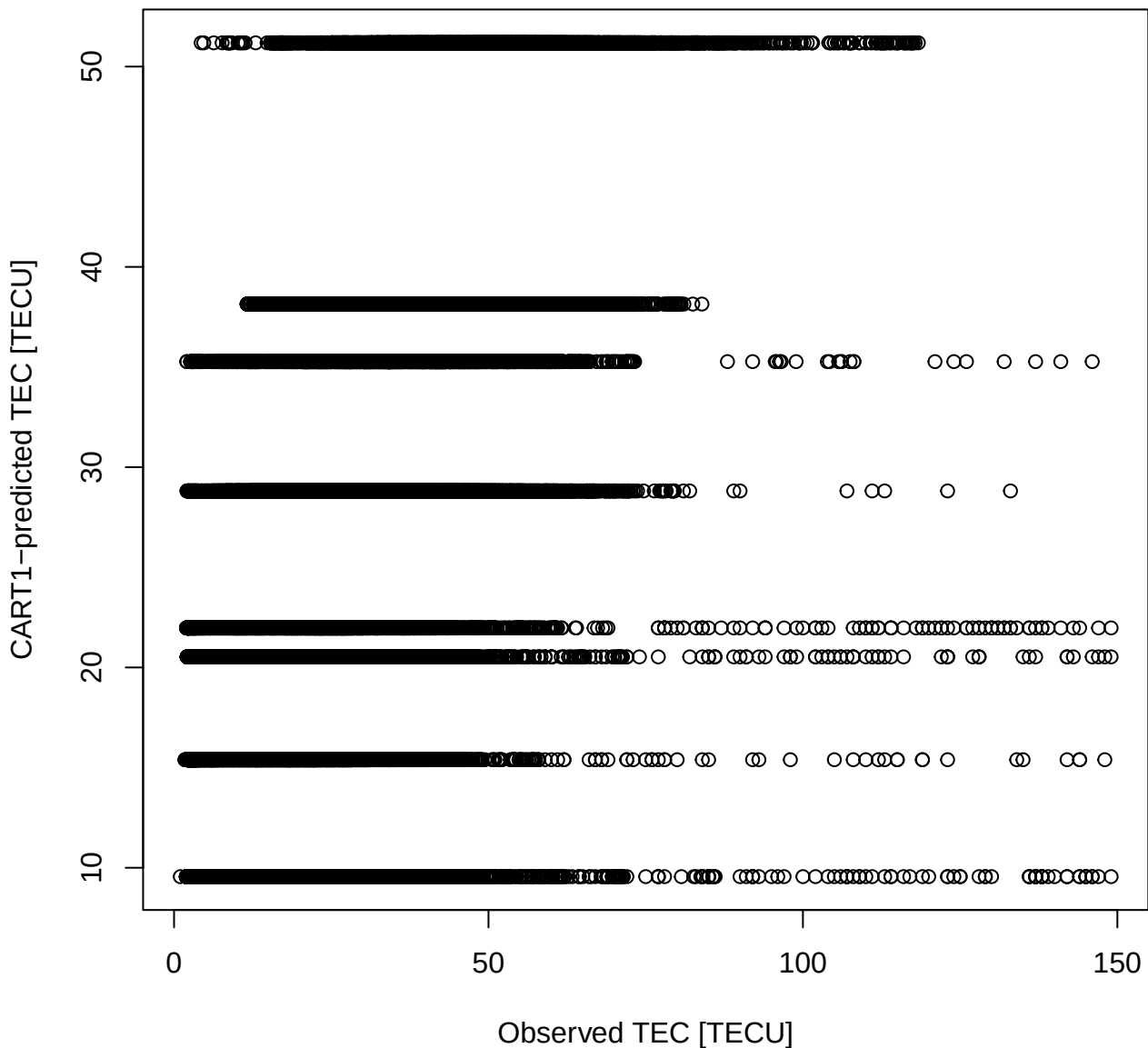
Observed and CART1-predicted TEC [TECU]
