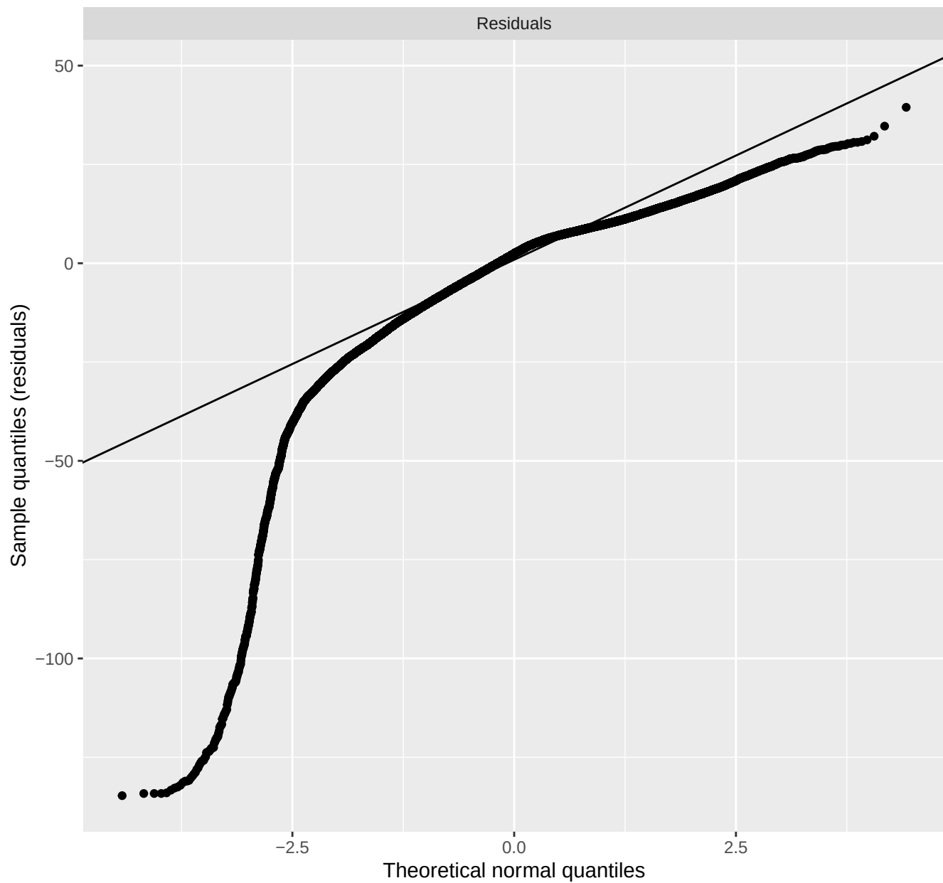
Q-Q plot for GAMB residuals
