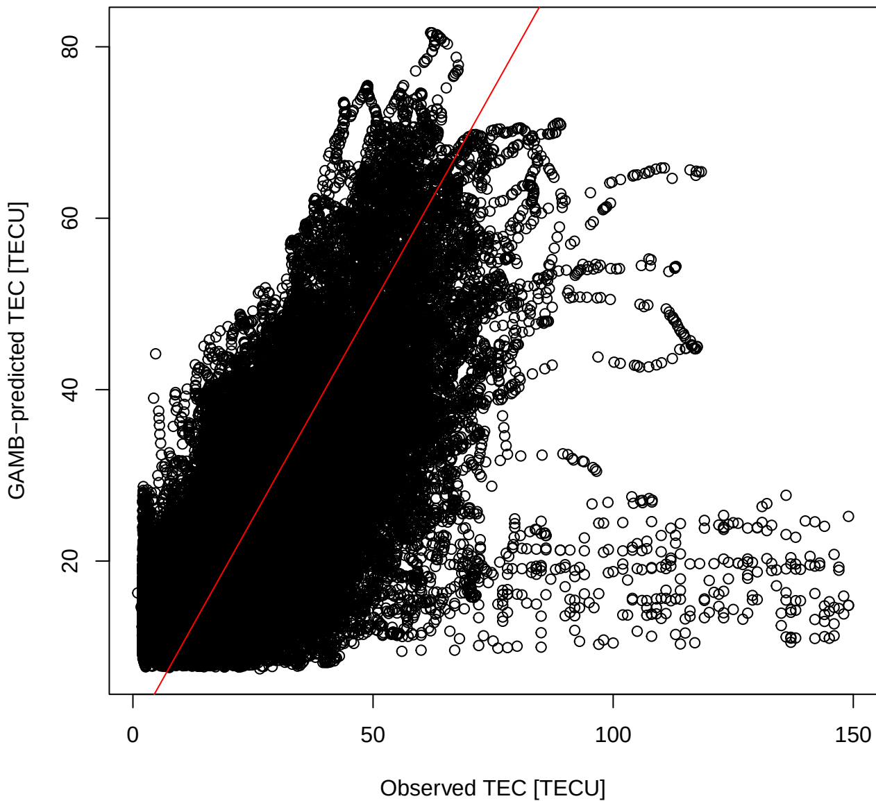
Observed and GAMB-predicted TEC [TECU]
