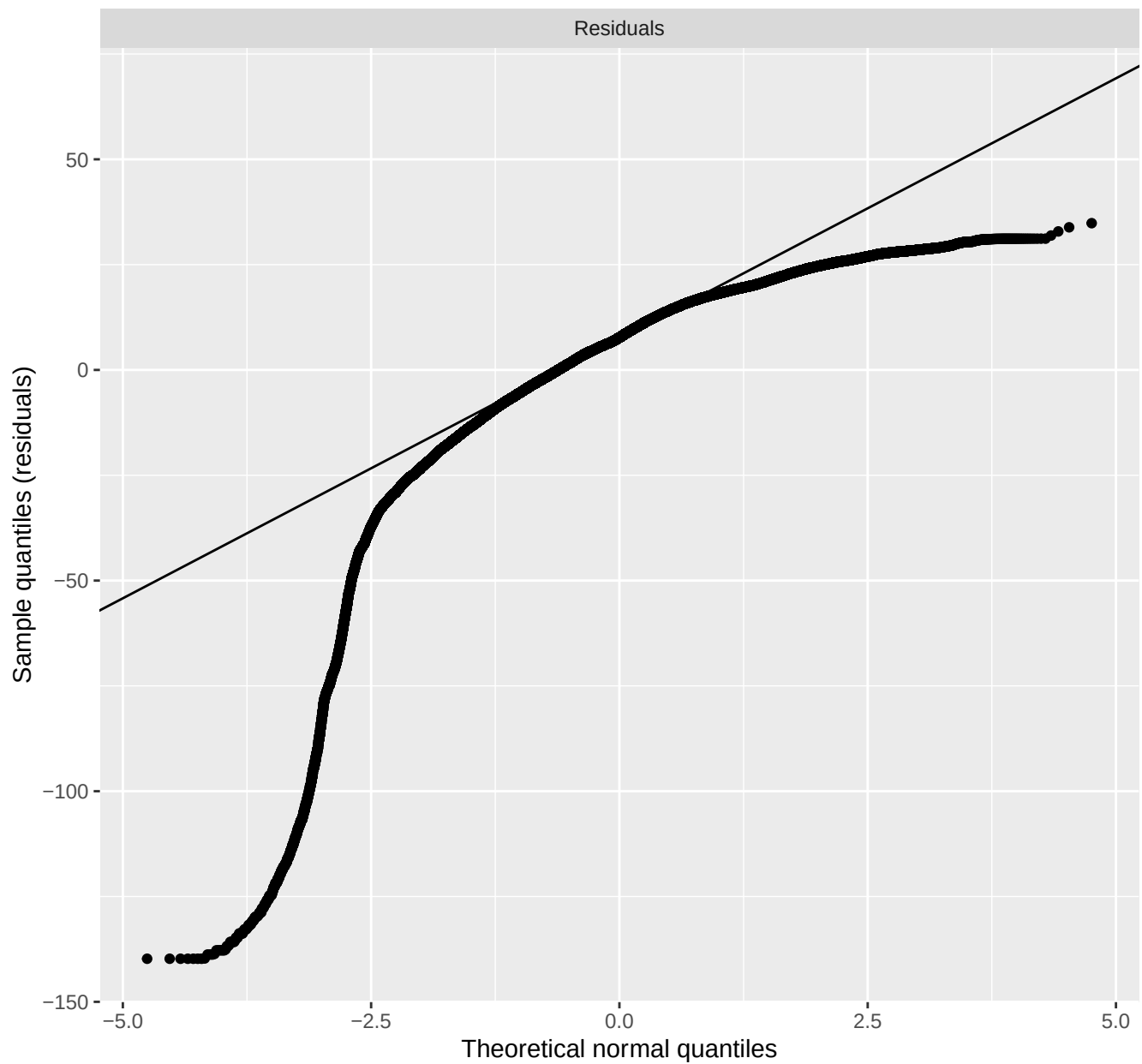
Q-Q plot for Klobuchar model residuals
