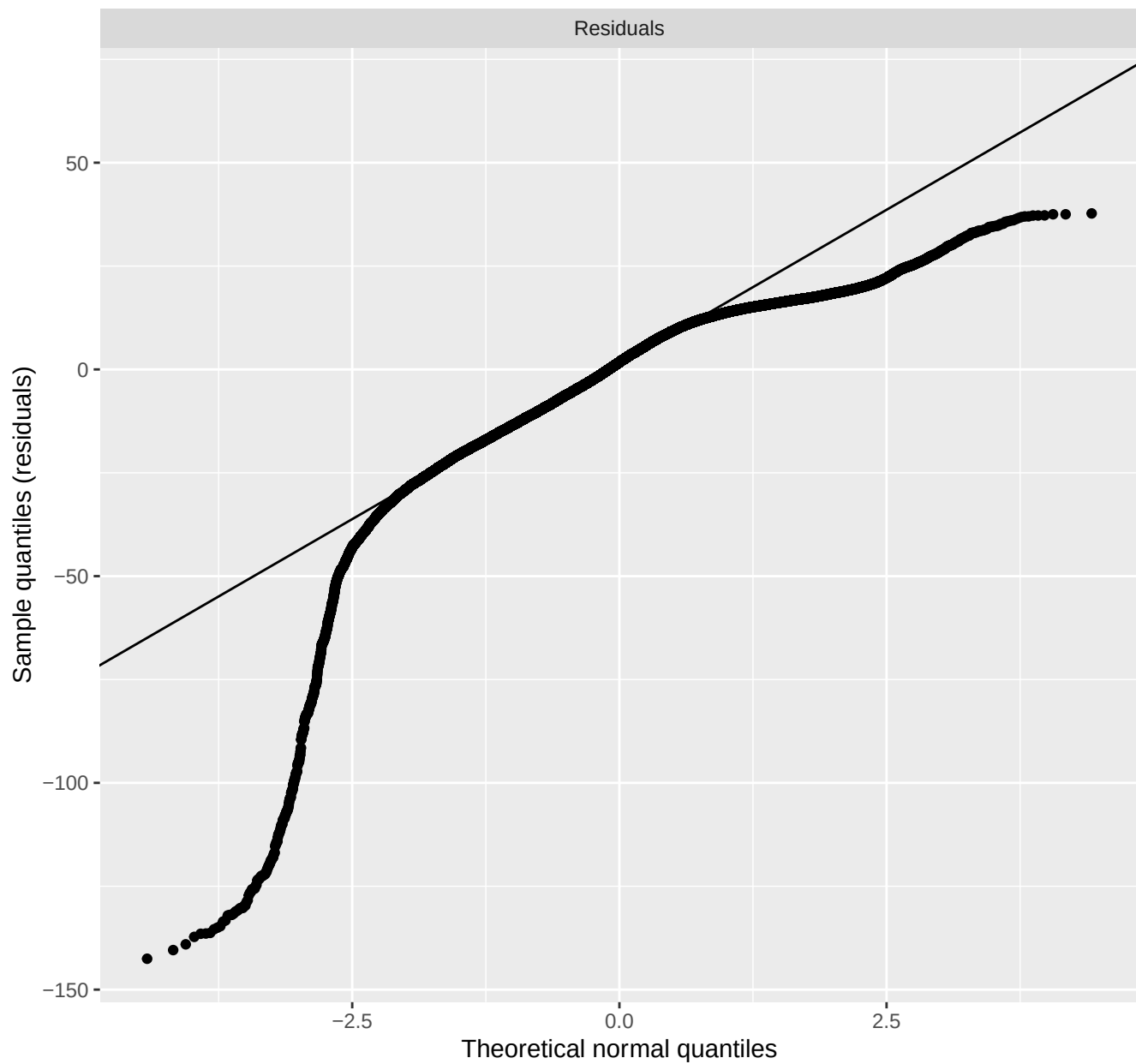
Q-Q plot for linear regression residuals
