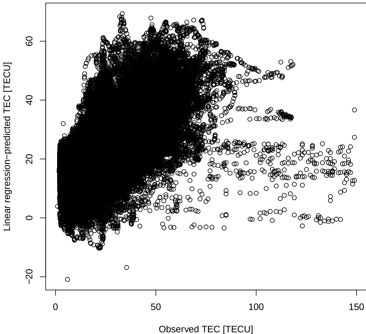
Observed and linear regression-predicted TEC [TECU]
