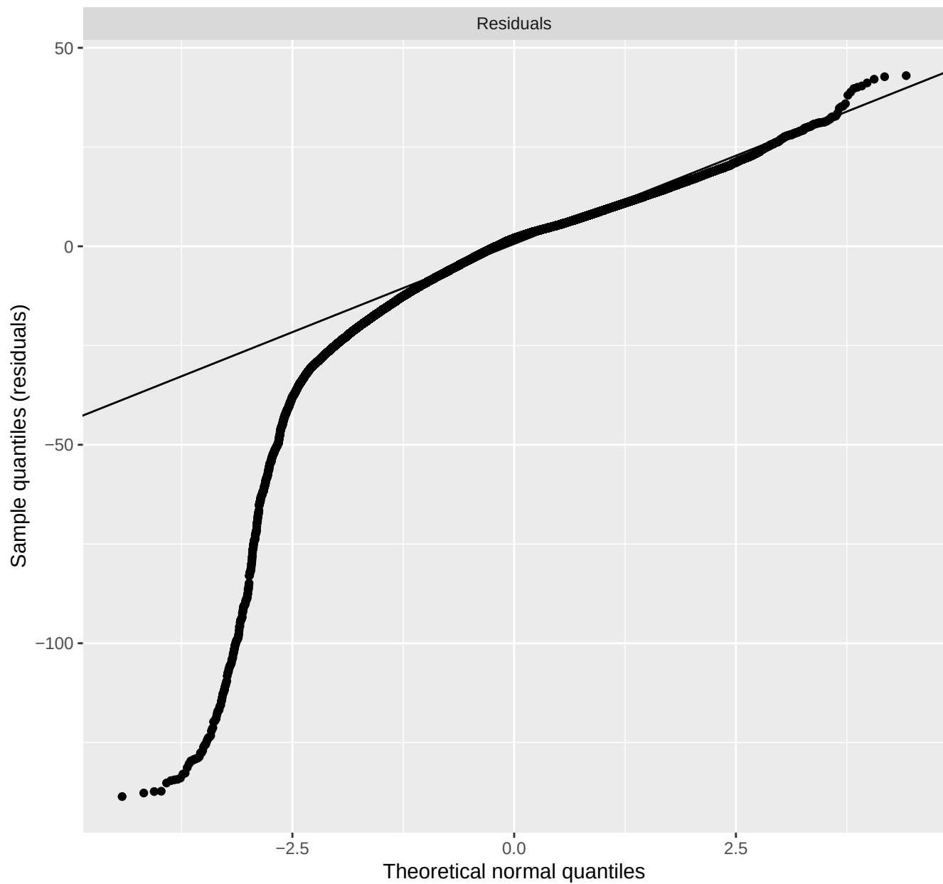
Q-Q plot for SGB residuals
