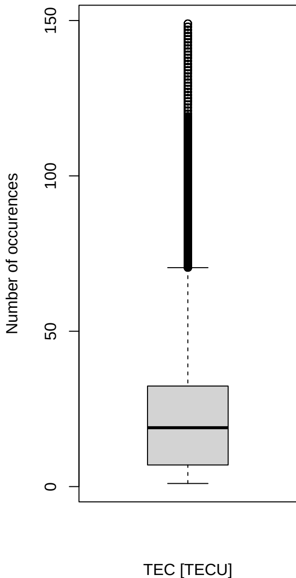
Number of occurrences TEC [TECU]
