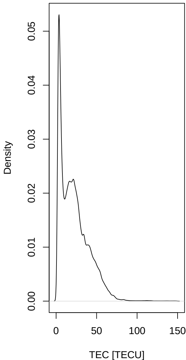
Probability density TEC [TECU]
