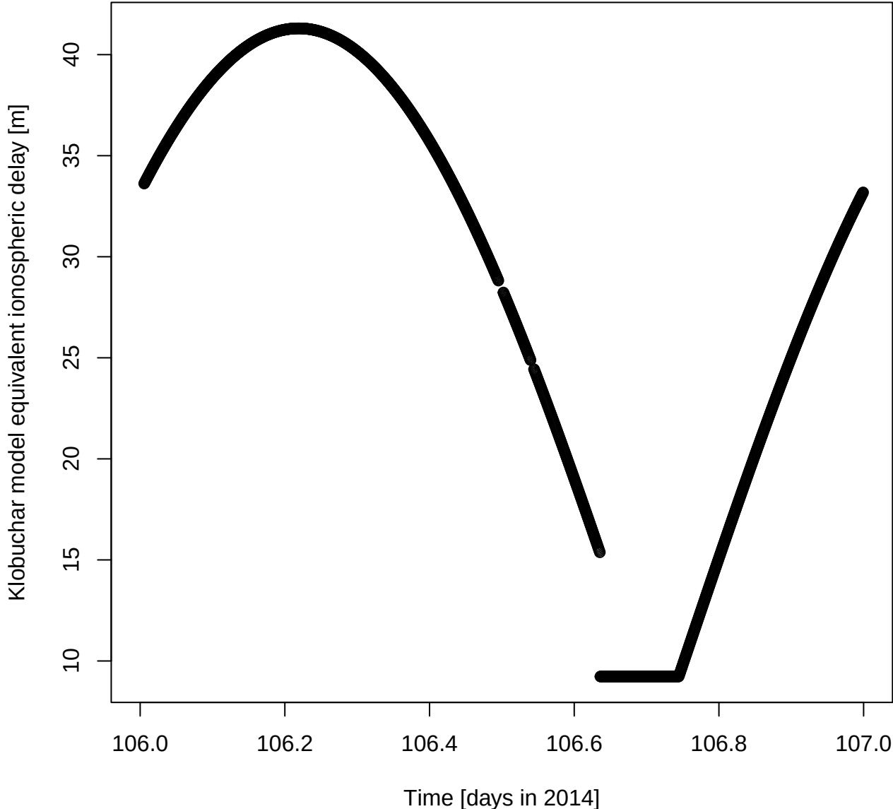
Klobuchar model equivalent ionospheric delay [m] for DOY 106 in 2014
