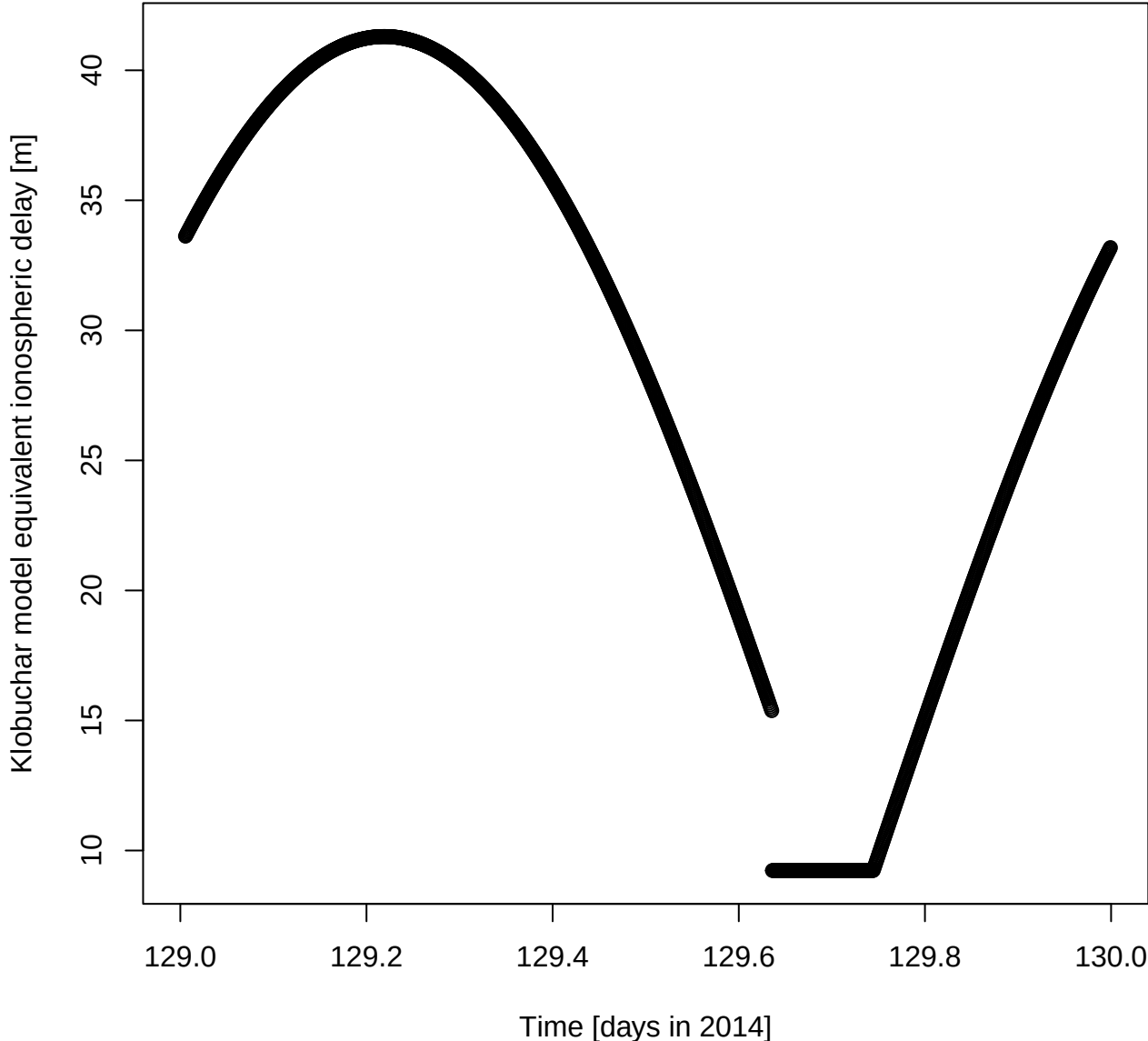
Klobuchar model equivalent ionospheric delay [m] for DOY 129 in 2014
