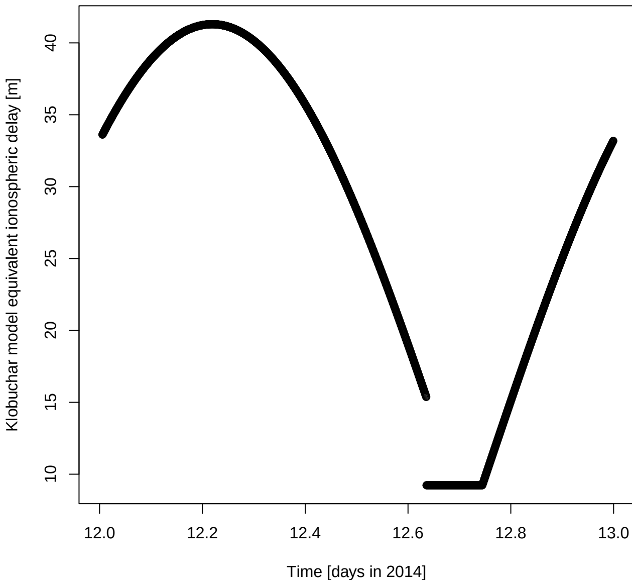
Klobuchar model equivalent ionospheric delay [m] for DOY 12 in 2014
