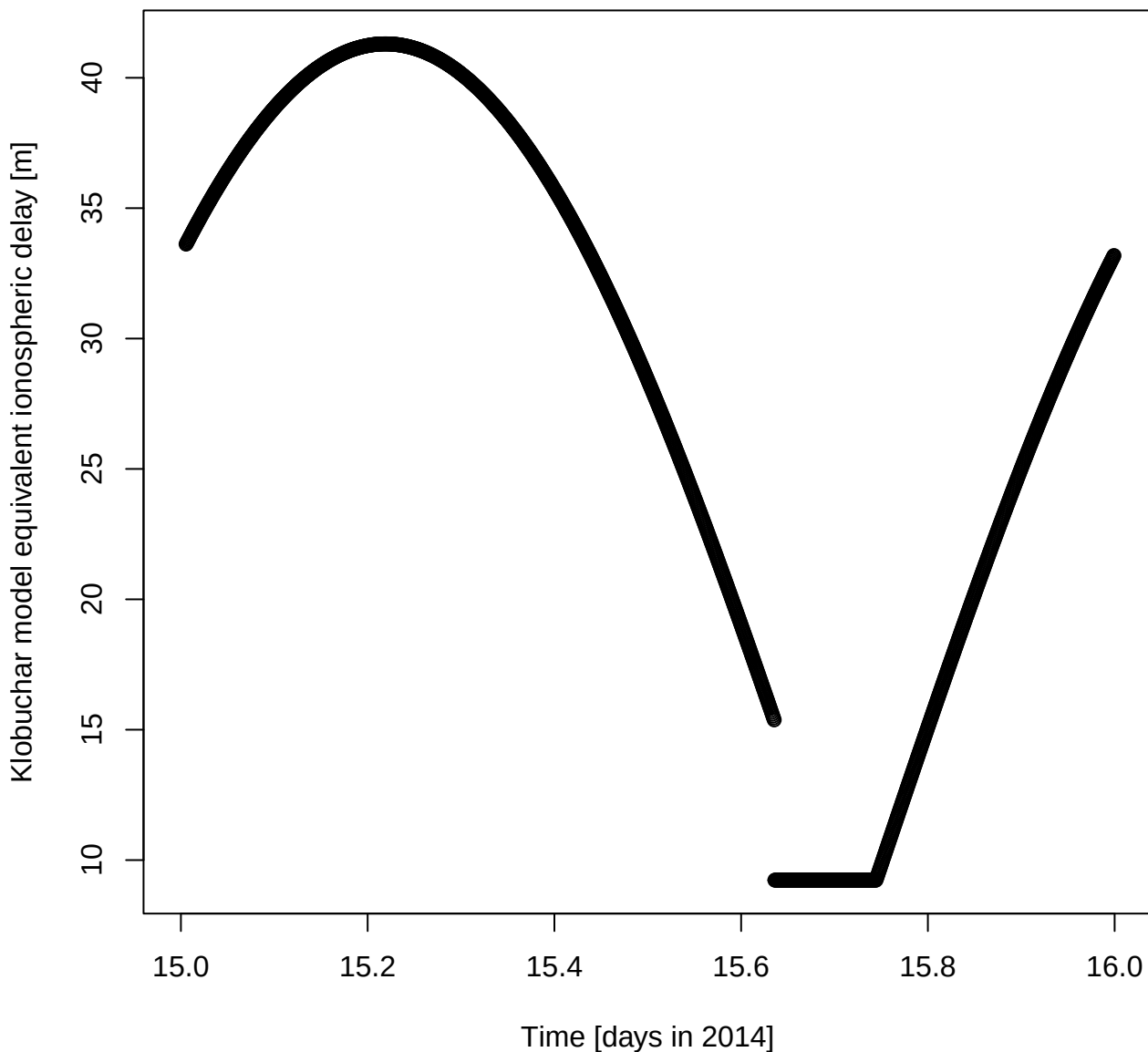
Klobuchar model equivalent ionospheric delay [m] for DOY 15 in 2014
