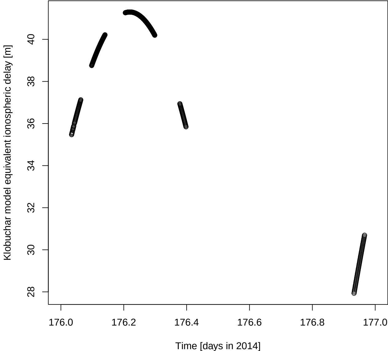
Klobuchar model equivalent ionospheric delay [m] for DOY 176 in 2014
