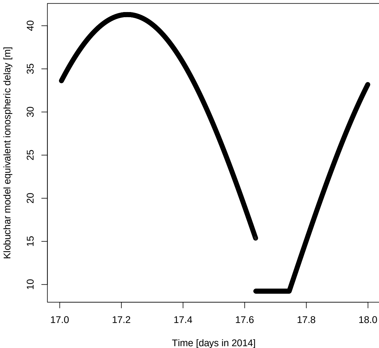
Klobuchar model equivalent ionospheric delay [m] for DOY 17 in 2014
