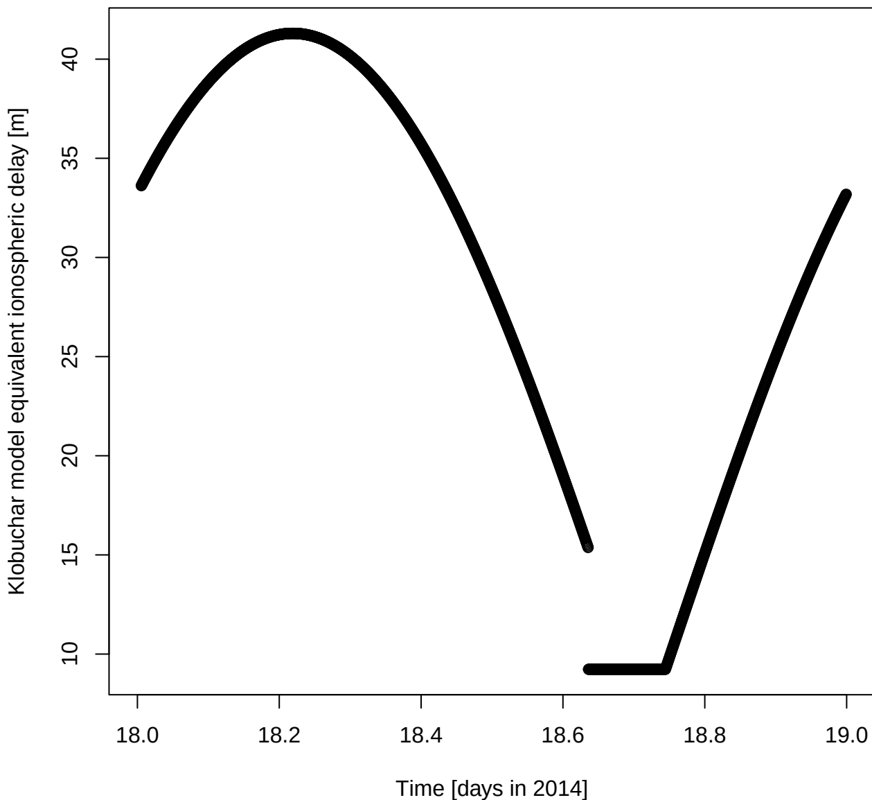
Klobuchar model equivalent ionospheric delay [m] for DOY 18 in 2014
