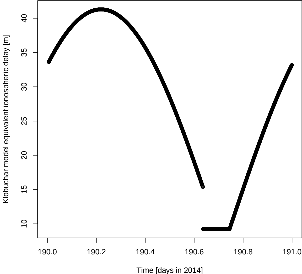
Klobuchar model equivalent ionospheric delay [m] for DOY 190 in 2014
