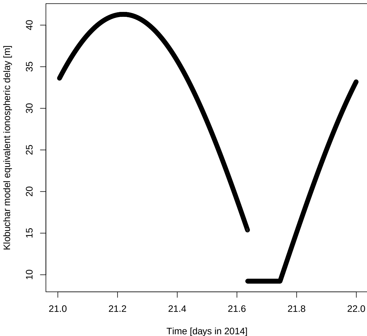
Klobuchar model equivalent ionospheric delay [m] for DOY 21 in 2014
