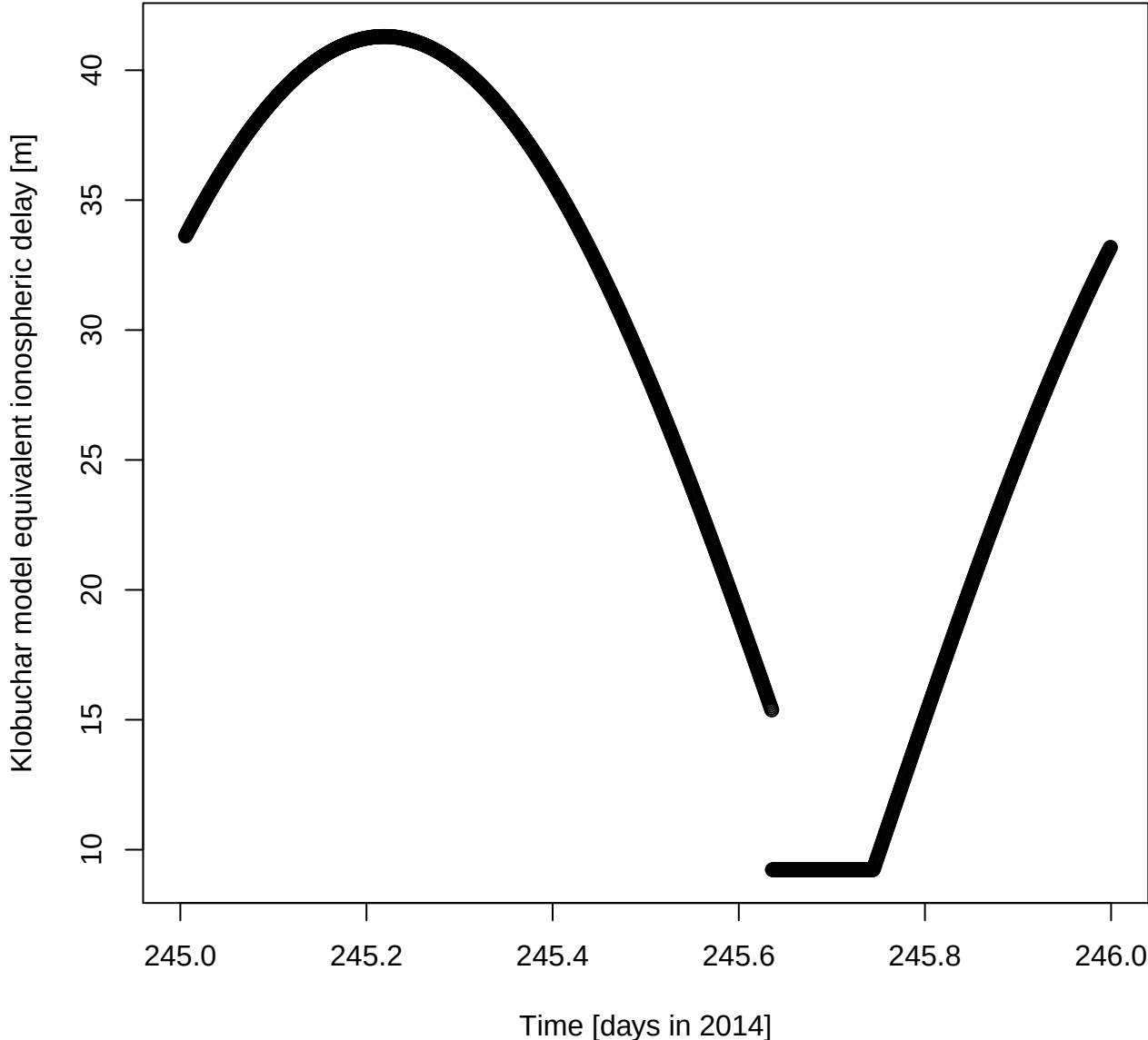
Klobuchar model equivalent ionospheric delay [m] for DOY 245 in 2014
