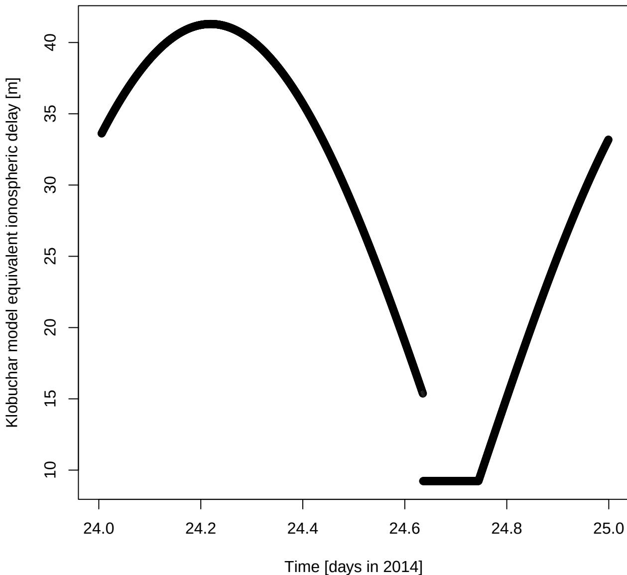
Klobuchar model equivalent ionospheric delay [m] for DOY 24 in 2014
