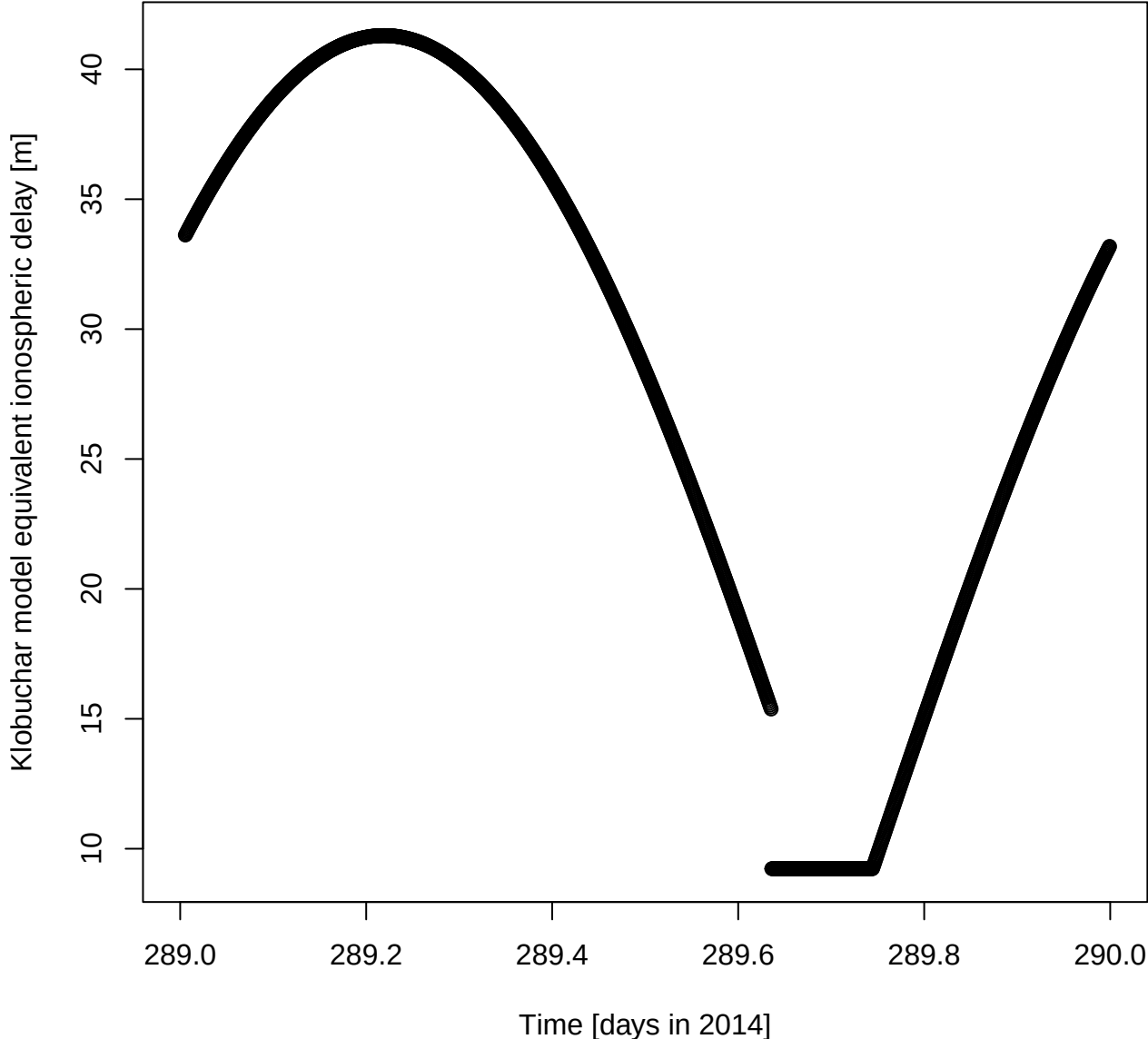
Klobuchar model equivalent ionospheric delay [m] for DOY 289 in 2014
