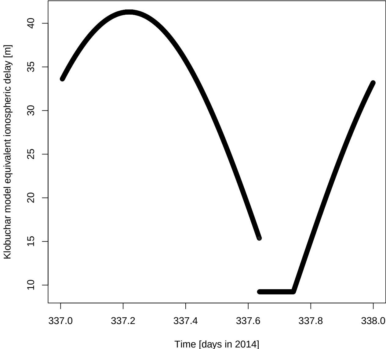
Klobuchar model equivalent ionospheric delay [m] for DOY 337 in 2014
