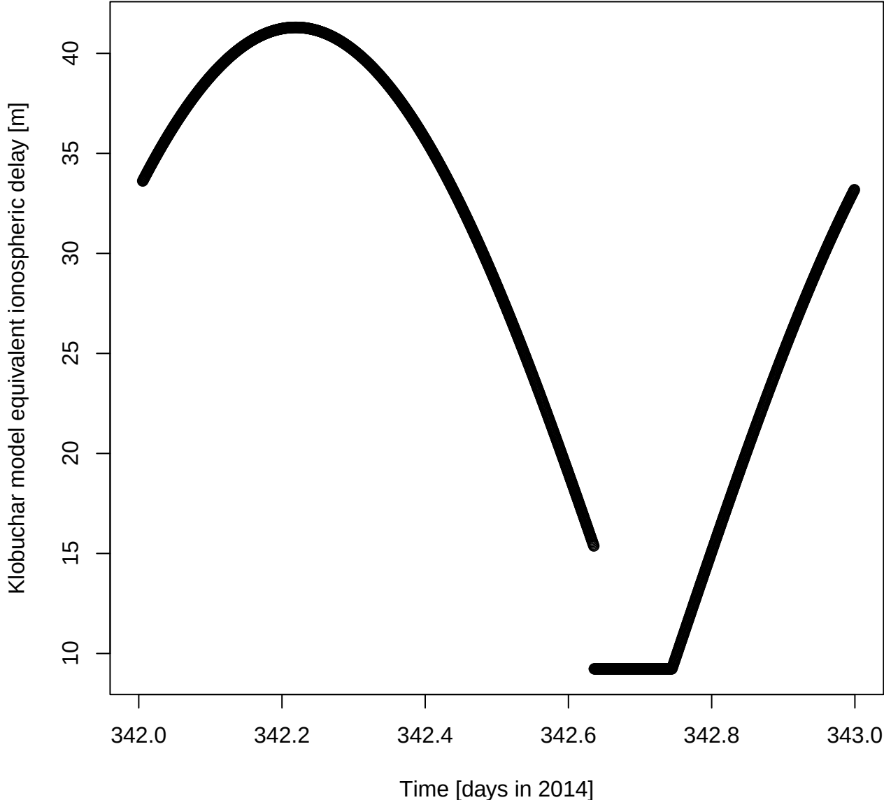
Klobuchar model equivalent ionospheric delay [m] for DOY 342 in 2014
