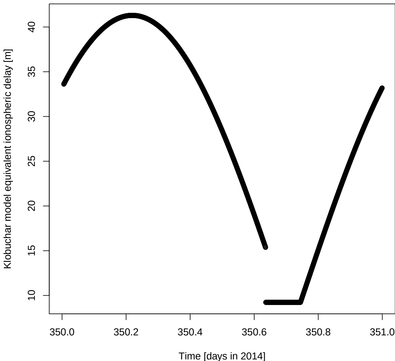
Klobuchar model equivalent ionospheric delay [m] for DOY 350 in 2014
