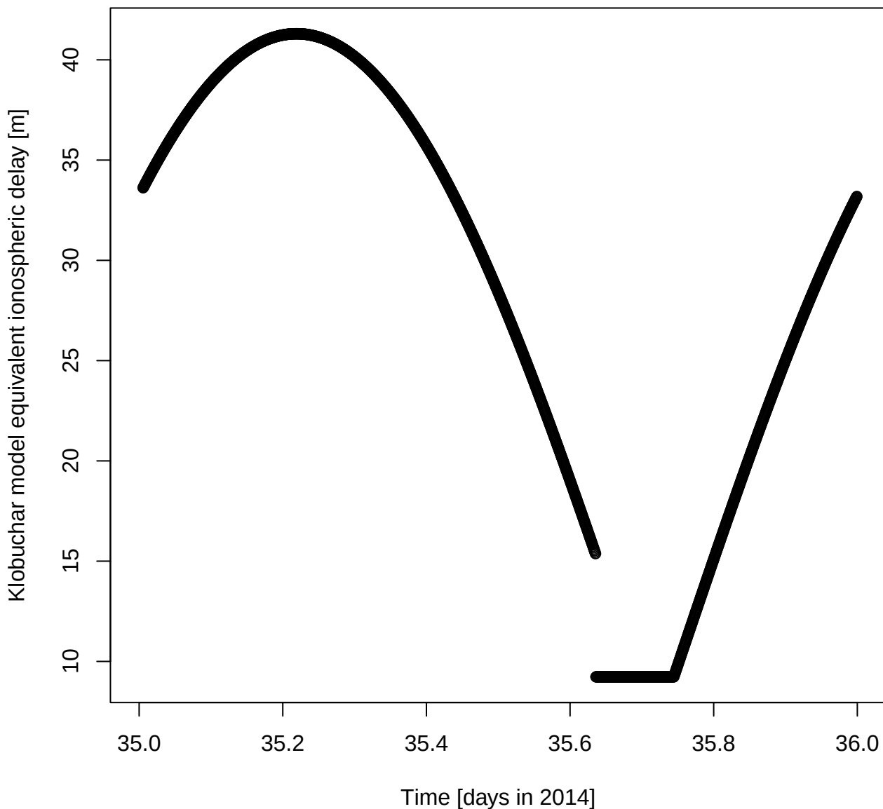
Klobuchar model equivalent ionospheric delay [m] for DOY 35 in 2014
