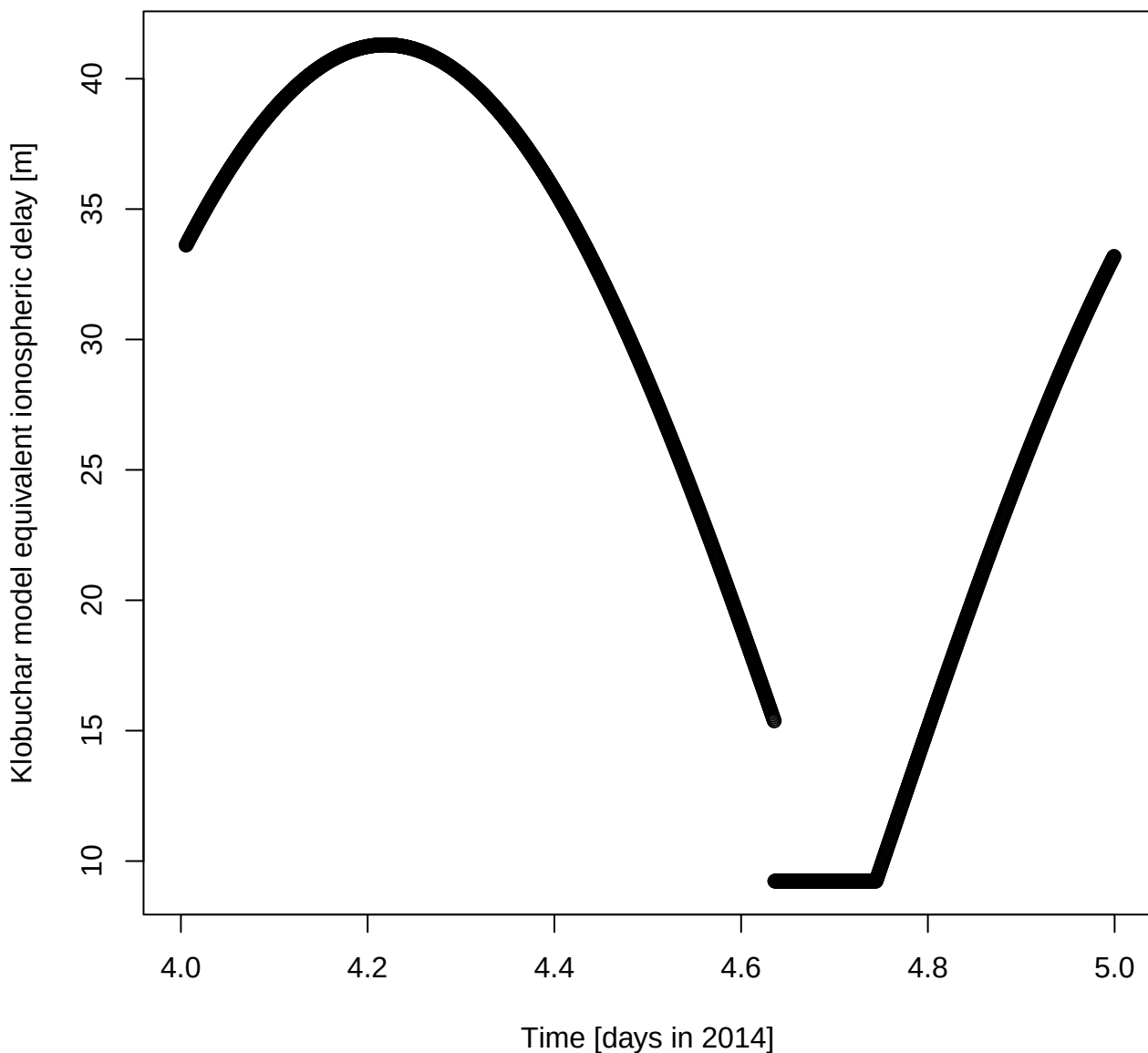
Klobuchar model equivalent ionospheric delay [m] for DOY 4 in 2014
