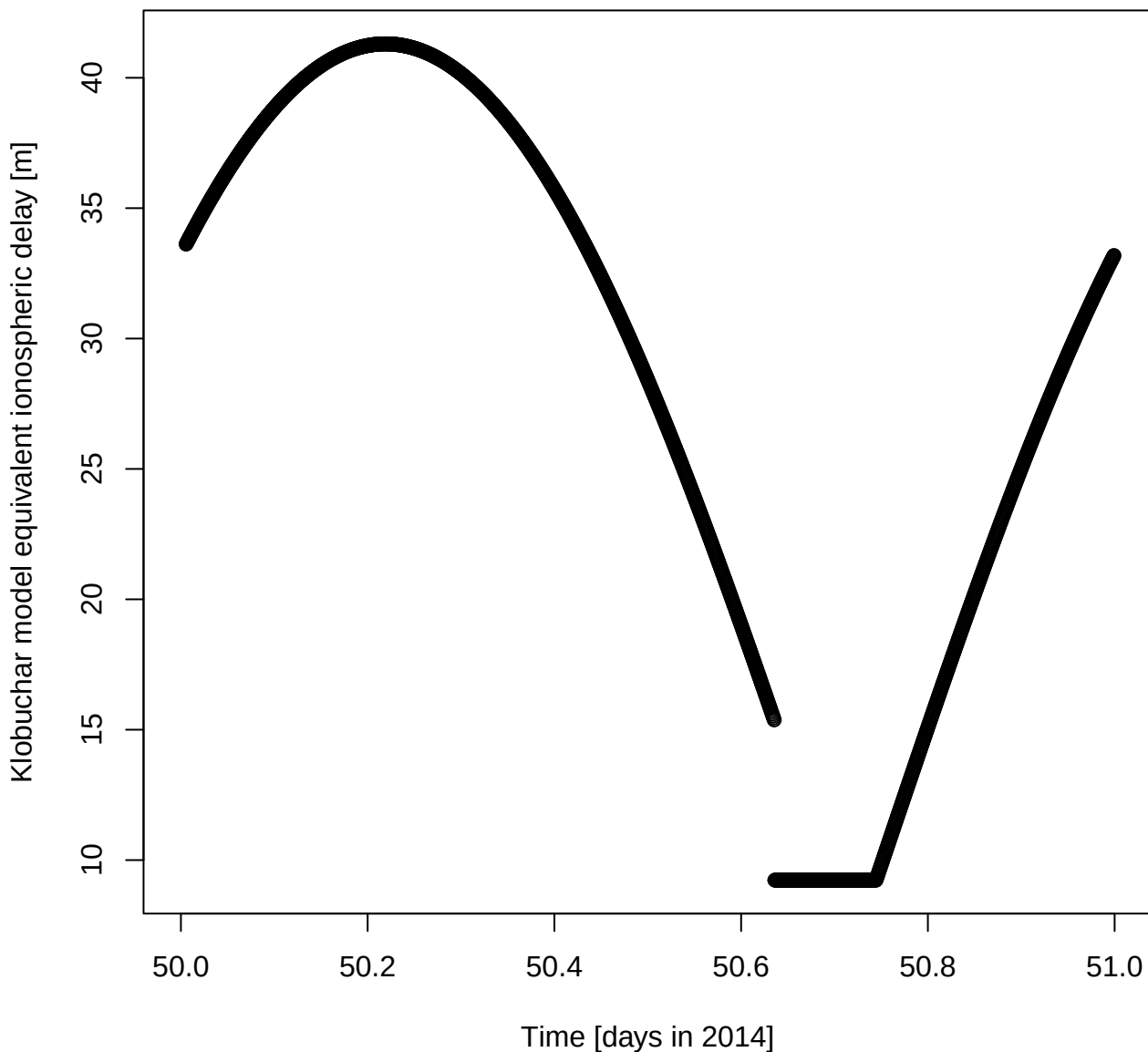
Klobuchar model equivalent ionospheric delay [m] for DOY 50 in 2014
