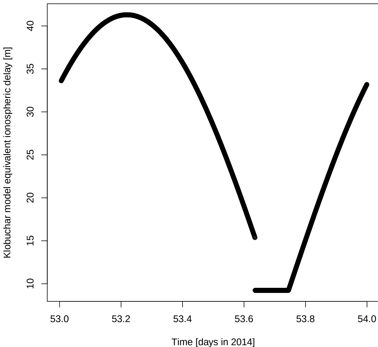
Klobuchar model equivalent ionospheric delay [m] for DOY 53 in 2014
