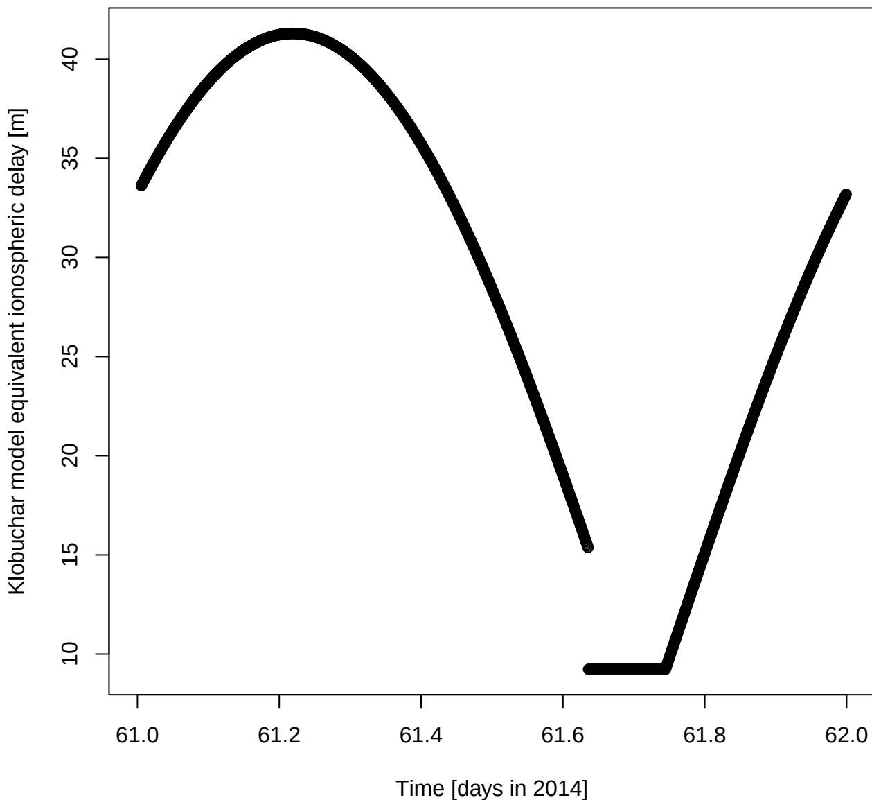
Klobuchar model equivalent ionospheric delay [m] for DOY 61 in 2014
