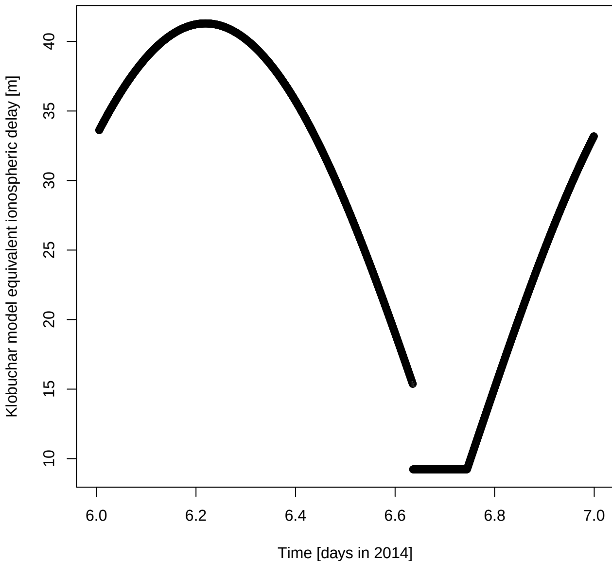
Klobuchar model equivalent ionospheric delay [m] for DOY 6 in 2014
