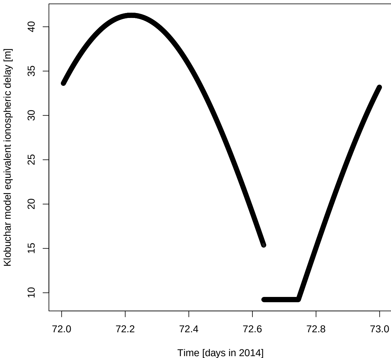
Klobuchar model equivalent ionospheric delay [m] for DOY 72 in 2014
