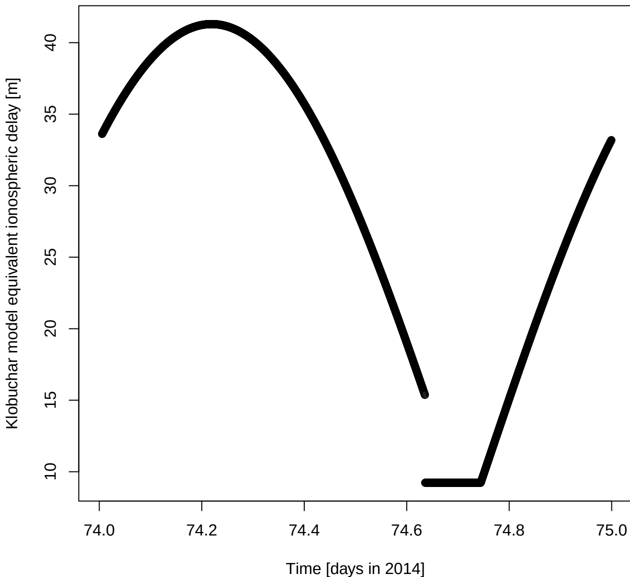
Klobuchar model equivalent ionospheric delay [m] for DOY 74 in 2014
