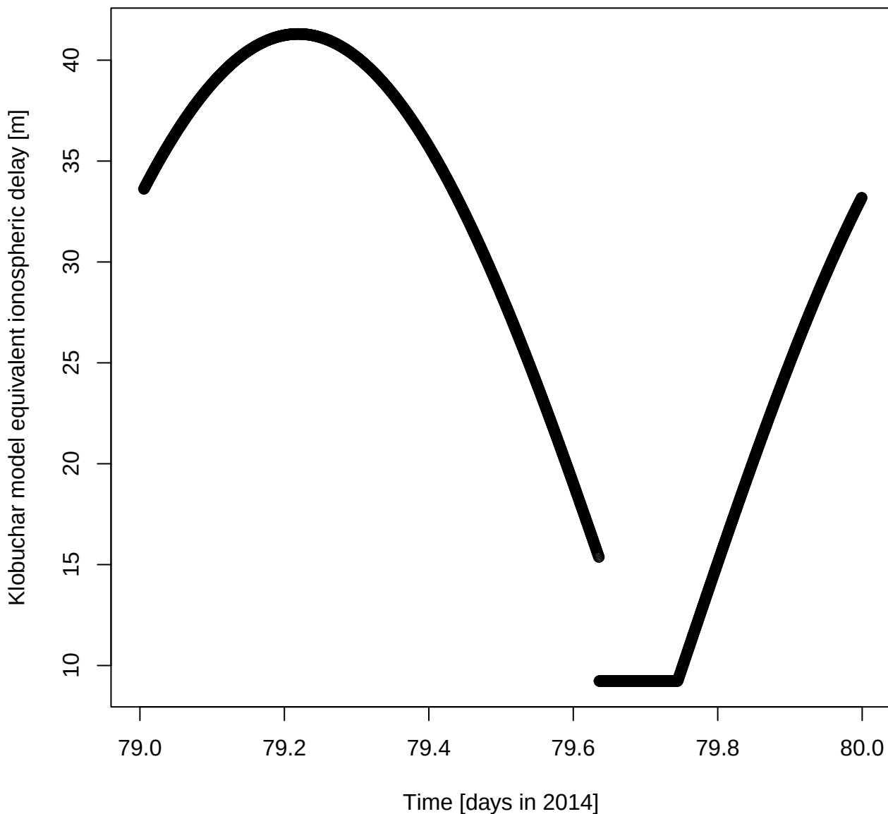
Klobuchar model equivalent ionospheric delay [m] for DOY 79 in 2014
