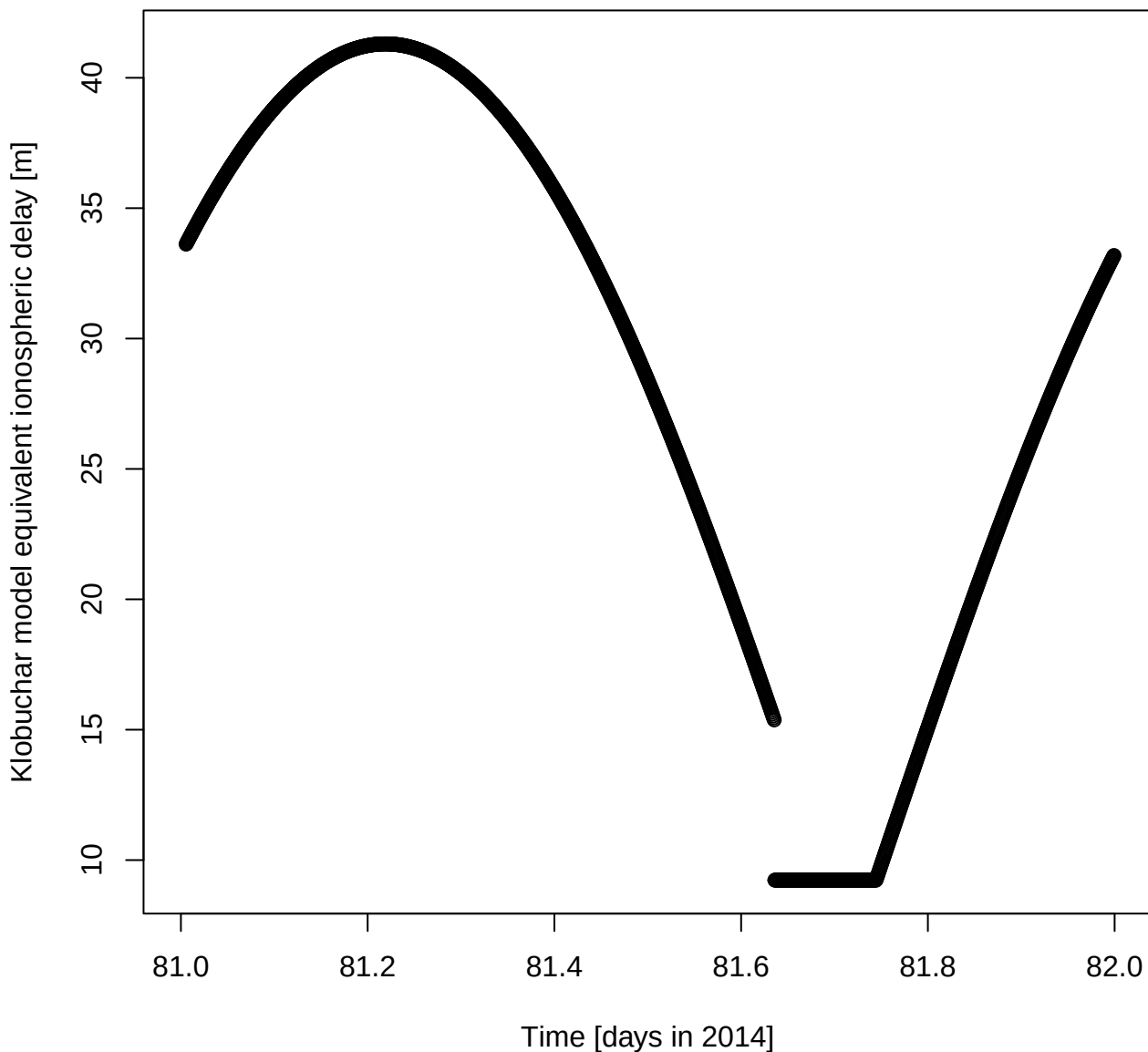
Klobuchar model equivalent ionospheric delay [m] for DOY 81 in 2014
