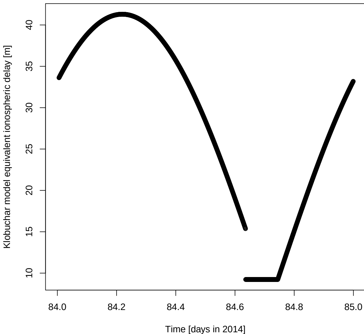
Klobuchar model equivalent ionospheric delay [m] for DOY 84 in 2014
