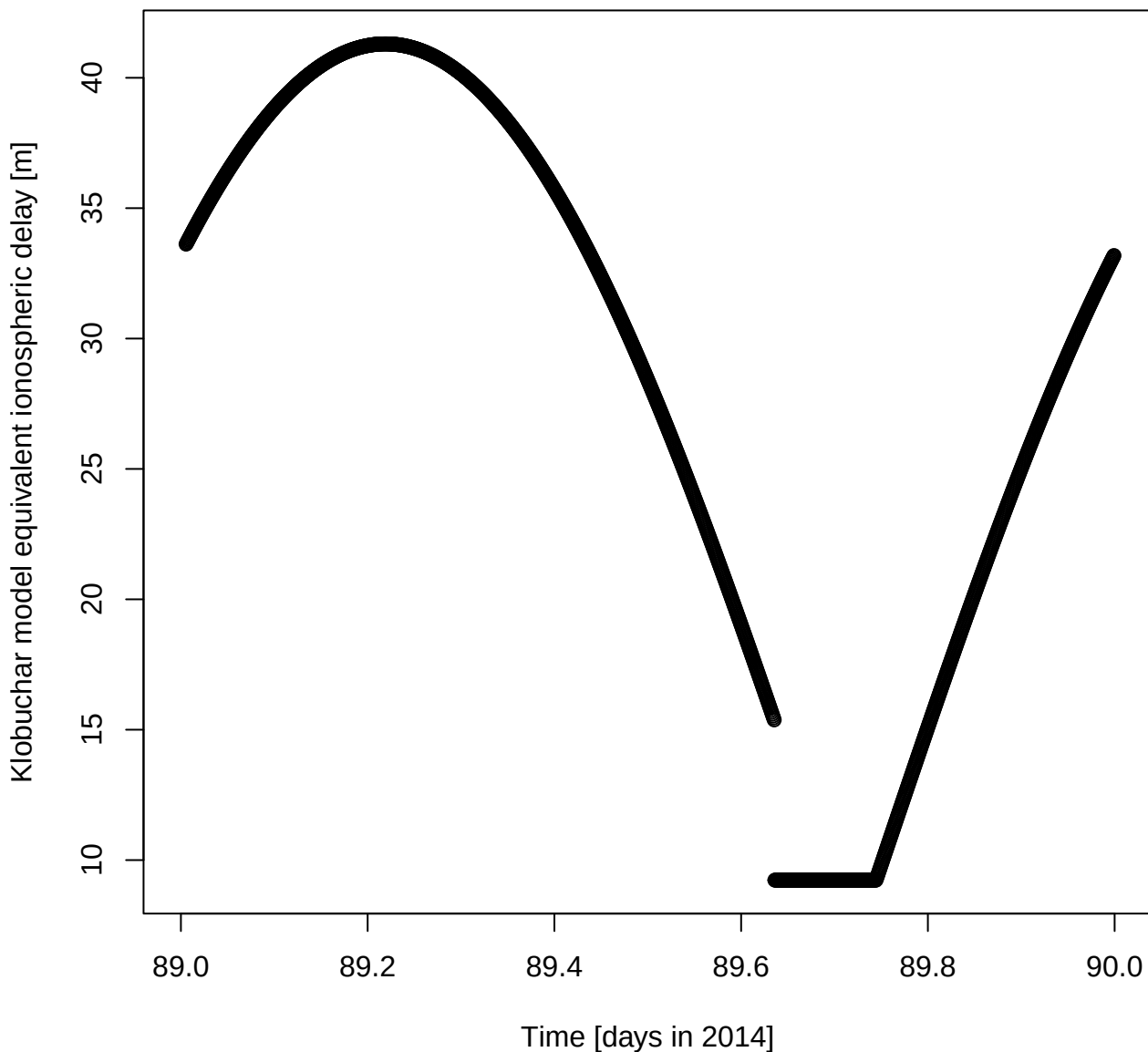
Klobuchar model equivalent ionospheric delay [m] for DOY 89 in 2014
