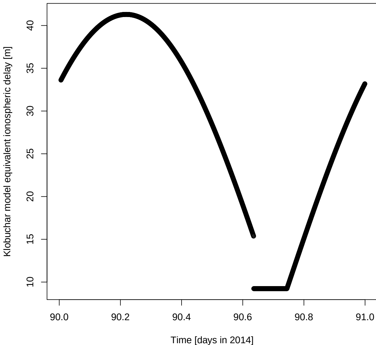
Klobuchar model equivalent ionospheric delay [m] for DOY 90 in 2014
