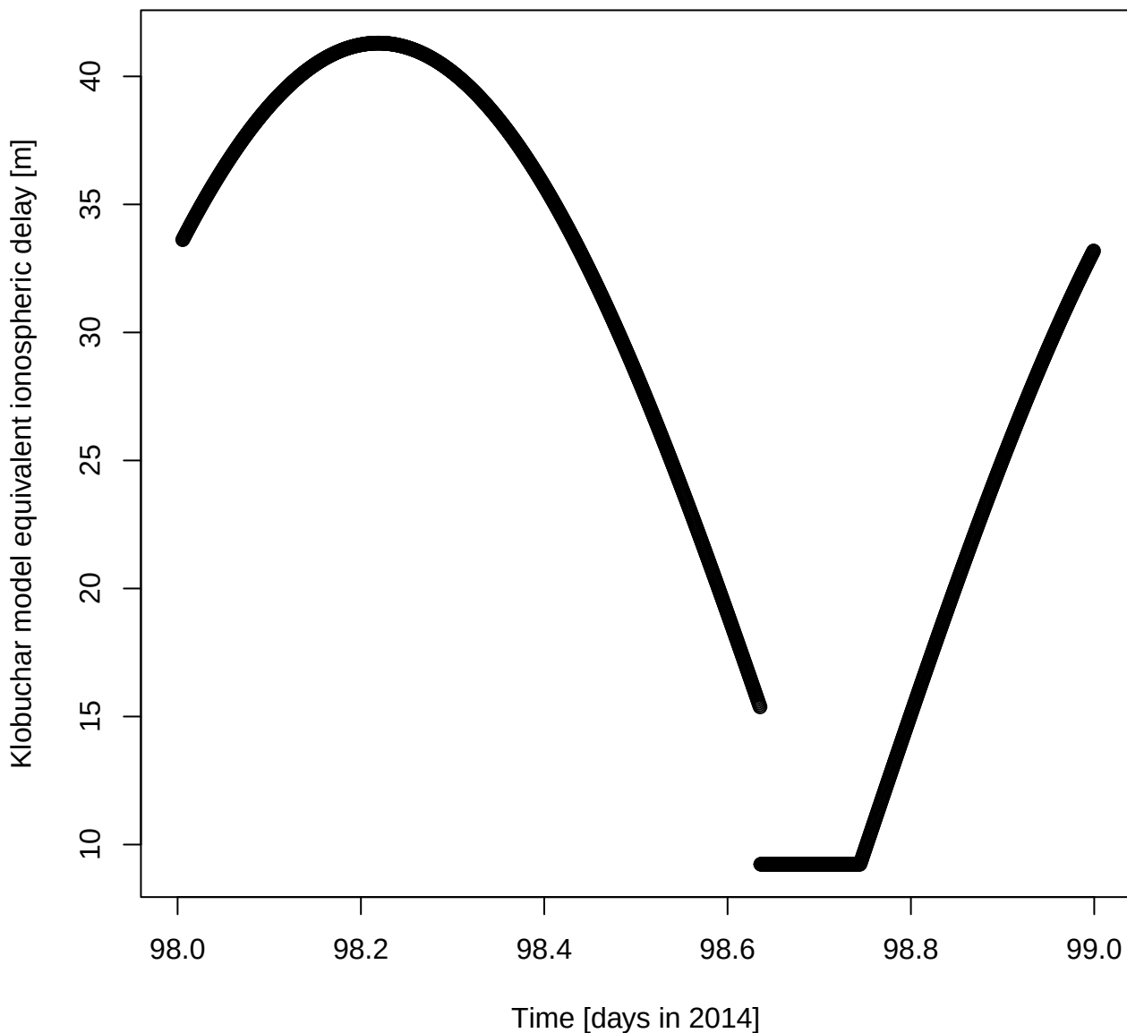
Klobuchar model equivalent ionospheric delay [m] for DOY 98 in 2014
