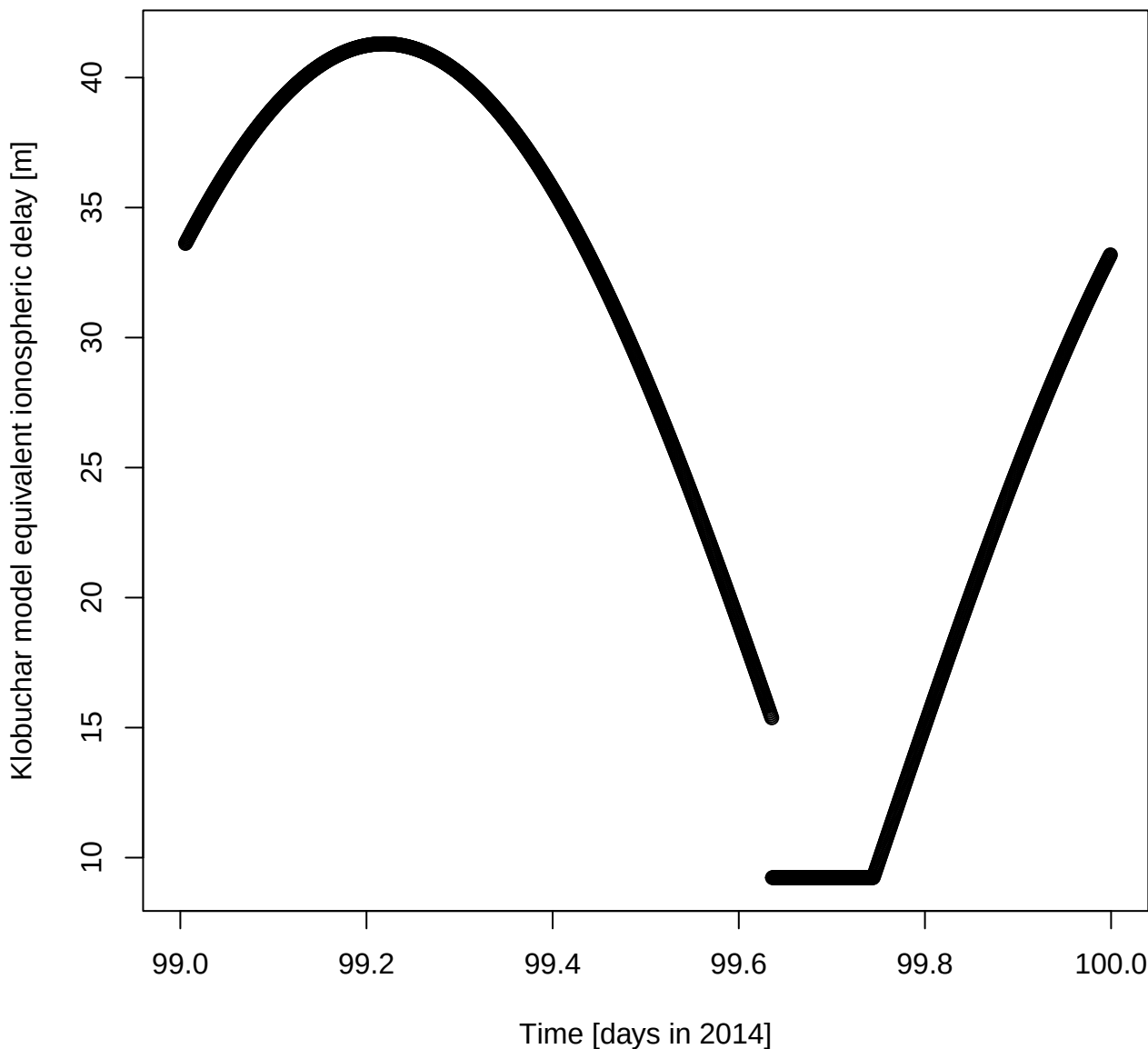
Klobuchar model equivalent ionospheric delay [m] for DOY 99 in 2014
