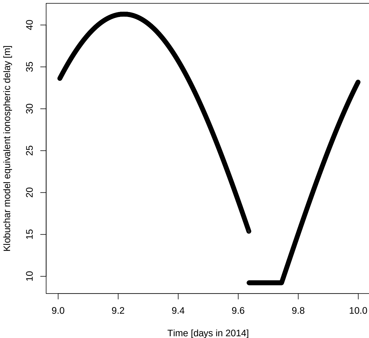
Klobuchar model equivalent ionospheric delay [m] for DOY 9 in 2014
