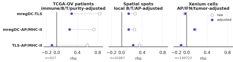
Supplementary Figure S6 Immune-richness-adjusted specificity audit. A , Raw and immune/B/T-cell/tumor-purity-adjusted Spearman correlations for mregDC-TLS, mregDC-AP/MHC-II, and TLS-AP/MHC-II associations in TCGA-OV patients. B , Raw and local B/T/AP-adjusted correlations for the same relationships across spatial transcriptomic spots. C , Raw and AP/IFN/tumor-adjusted correlations in Xenium cells.
