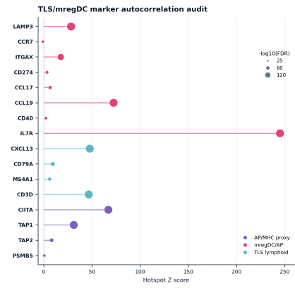
Supplementary Figure S2 Hotspot spatial-autocorrelation audit. A, Top spatially autocorrelated genes ranked by Hotspot Z score in sampled Xenium cells. B, Marker-level Hotspot audit for TLS/mregDC/AP-associated genes, grouped by AP/MHC-II proxy, mregDC/AP, and TLS lymphoid marker categories.
