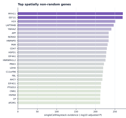
Supplementary Figure S1 singleCellHaystack spatial non-randomness audit. A , Top spatially non-random genes ranked by singleCellHaystack evidence in the deterministic ovarian cancer subset. B , Marker-level audit for TLS/mregDC/AP-associated genes, grouped by AP/MHC-II proxy, mregDC/AP, and TLS lymphoid marker categories.
