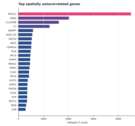
Supplementary Figure S2 Hotspot spatial-autocorrelation audit. A, Top spatially autocorrelated genes ranked by Hotspot Z score in sampled Xenium cells. B, Marker-level Hotspot audit for TLS/mregDC/AP-associated genes, grouped by AP/MHC-II proxy, mregDC/AP, and TLS lymphoid marker categories.
