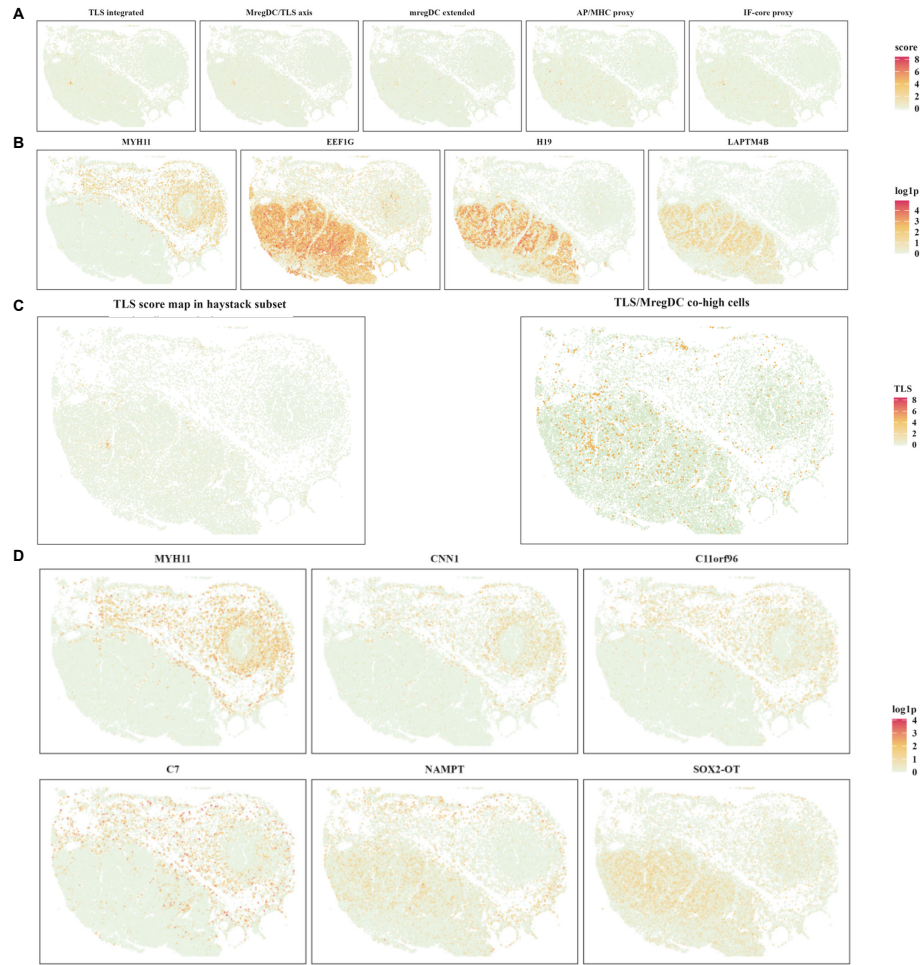
Supplementary Figure S3 Xenium spatial maps supporting feature audits. A , Spatial module maps for TLS-integrated, mregDC/TLS-axis, mregDC-extended, AP/MHC proxy, and IF-core proxy scores. B , Representative spatial expression maps for singleCellHaystack-prioritized non-random genes. C , TLS-score map and TLS/mregDC co-high cells in the same Xenium coordinate framework. D , Representative spatial expression maps for Hotspot-prioritized autocorrelated genes.
