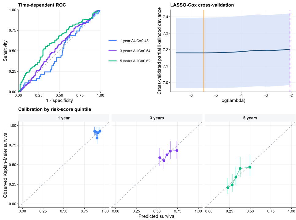
Supplementary Figure S5 Exploratory model validation. A , Time-dependent ROC curves for 1-, 3-, and 5-year internal model assessment in TCGA-OV. B , LASSO-Cox cross-validation curve with selected penalty marker. C , Calibration-by-risk-quintile summaries for 1-, 3-, and 5-year predicted survival.
