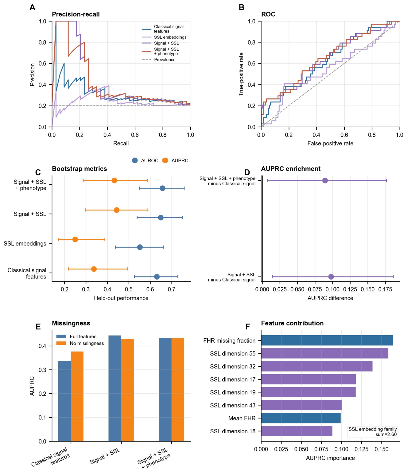
Figure 2. Self-supervised CTG representations are associated with risk enrichment and contribute measurable AI features. Held-out validation and explanation of neonatal risk prediction models in the CTU-UHB test set (34 events among 166 records). (A) Precision-recall curves comparing classical signal features, SSL embeddings, signal-plus-SSL, and signal-plus-SSL-plus-phenotype models. (B) Receiver-operating-characteristic curves for the same AI feature sets. (C) Bootstrap validation of AUROC and AUPRC; points show observed test-set estimates and whiskers show 95% bootstrap confidence intervals from 2,000 resamples. (D) Bootstrap AUPRC differences versus classical signal features; intervals approach zero, and the gain is not statistically secure once missingness features are removed. (E) Missingness sensitivity after removing FHR and UQ. (F) AUPRC-based permutation importance in the signal-plus-SSL model; SSL dimensions appear among the highest-ranking predictors and the SSL embedding family contributes substantial aggregate positive importance distributed across multiple dimensions. Estimates reflect a held-out-ranked configuration and should be interpreted as exploratory; the development only selection is reported as the more conservative enrichment
