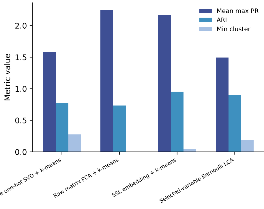
Phenotyping baseline comparison
