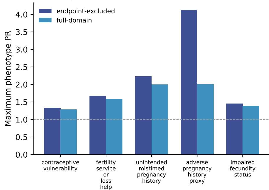
Endpoint-excluded vs full-domain encoder
