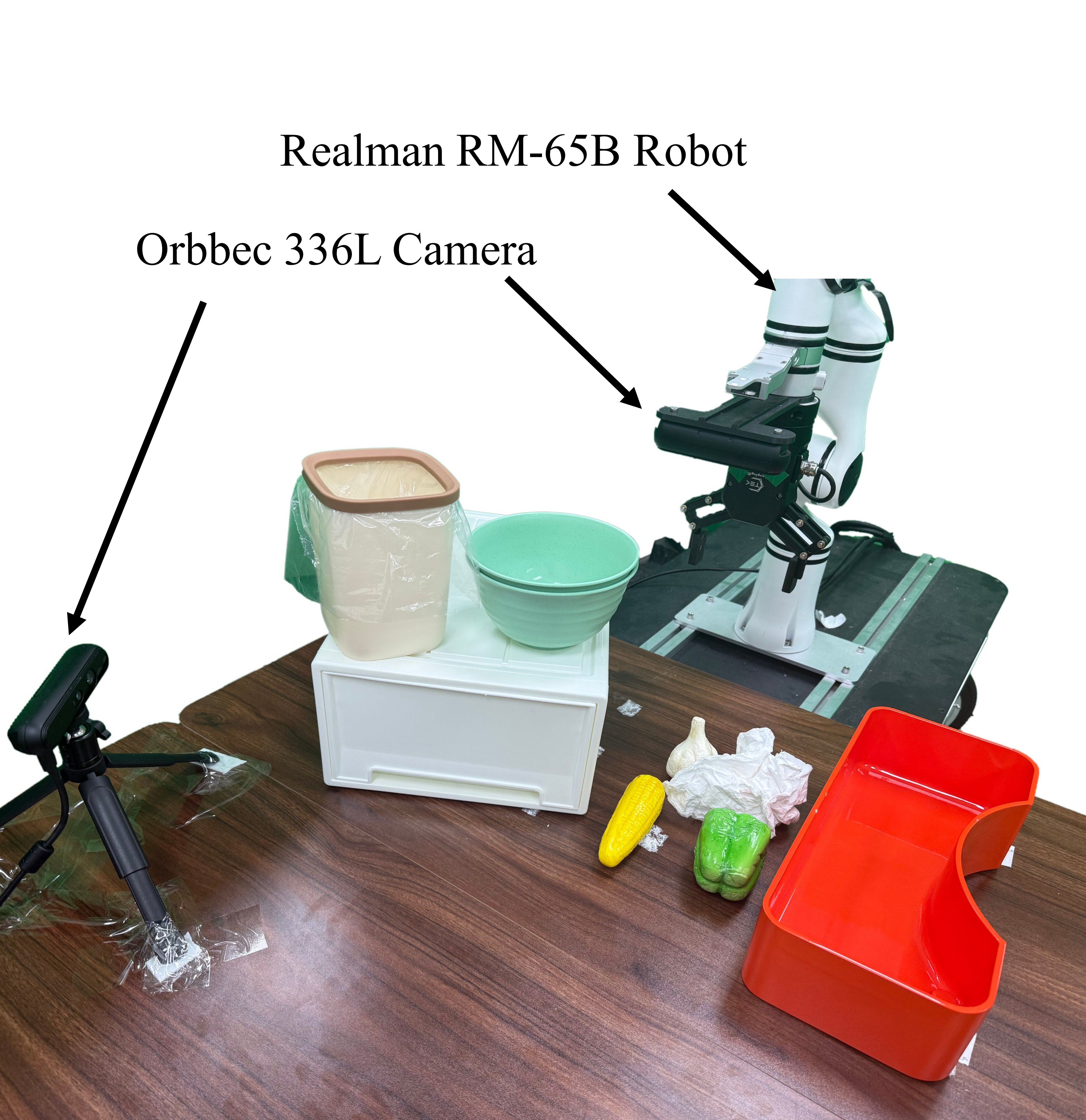
Experiment Hardware Setup
