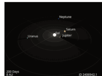
An animation of Saturn and the Solar System's outer planets orbiting the Sun
