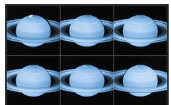
Auroral lights at Saturn's north pole
