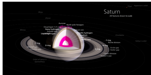
A diagram of Saturn, to scale
