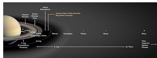
An artist conception of Saturn, its rings and major icy moons—from Mimas to Rhea
