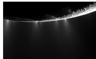
At Enceladus's south pole, geysers spray water from many locations along the tiger stripes . [165]
