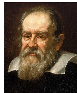
Galileo Galilei observed the rings of Saturn in 1610, but was unable to determine what they were.
