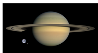
The size of Saturn, compared to Earth and its moon
