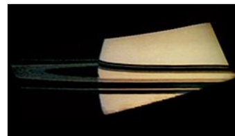
Pioneer 11 image of Saturn
