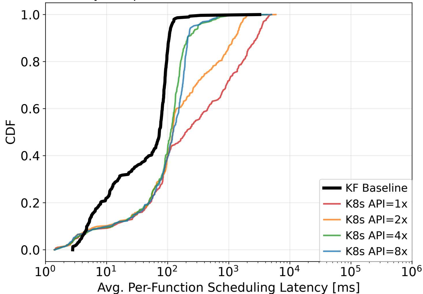
Latency Comparison: KF vs K8s with Different API Factors
