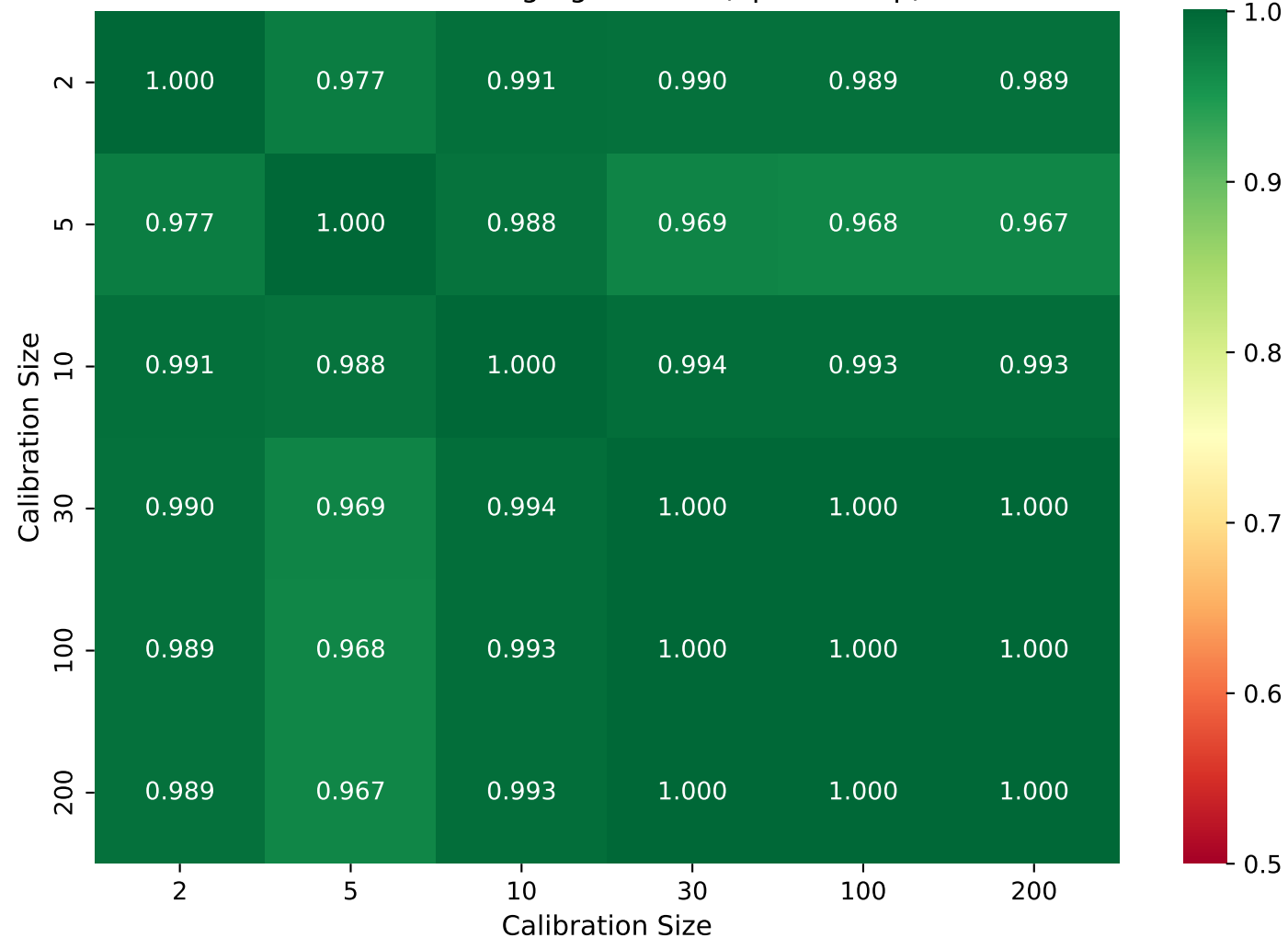
activation_l2_distance Pairwise Ranking Agreement (Spearman \rho )
