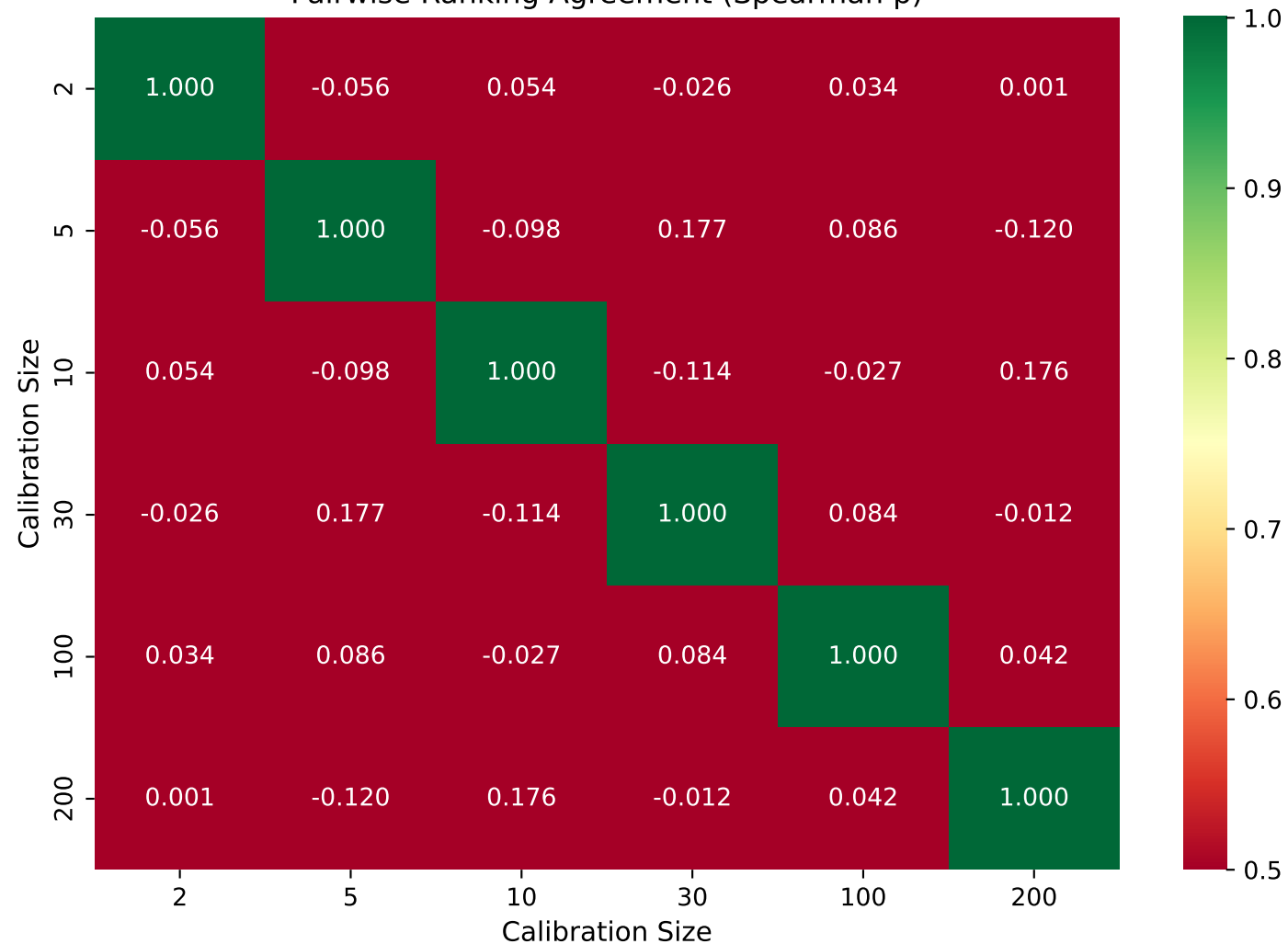
encoder_gradient_dot_product Pairwise Ranking Agreement (Spearman \rho )
