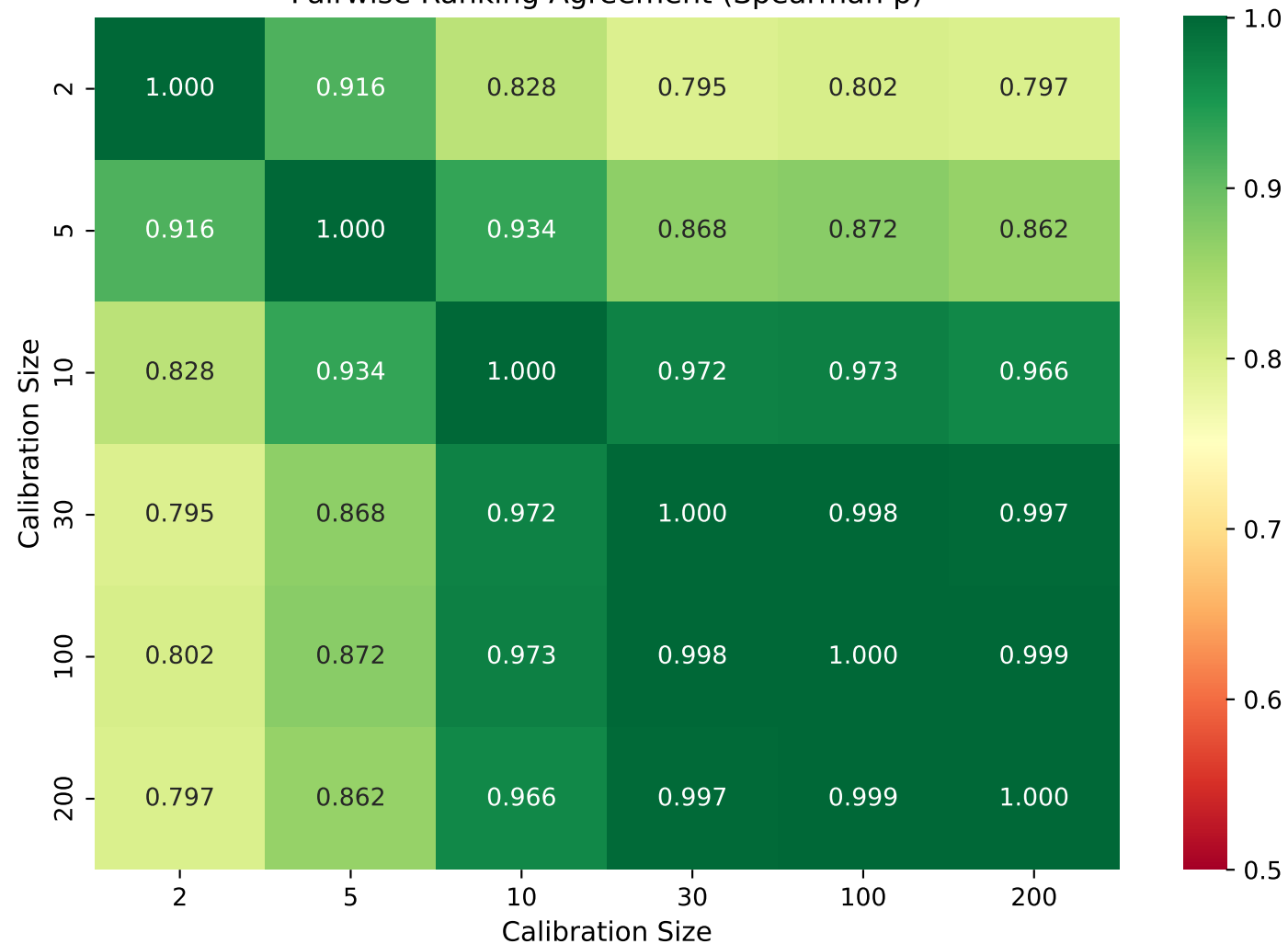
activation_magnitude_ratio Pairwise Ranking Agreement (Spearman \rho )
