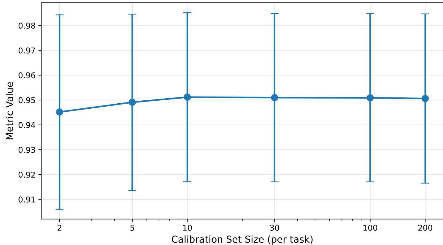
activation_magnitude_ratio Mean \pm Std across pairs
