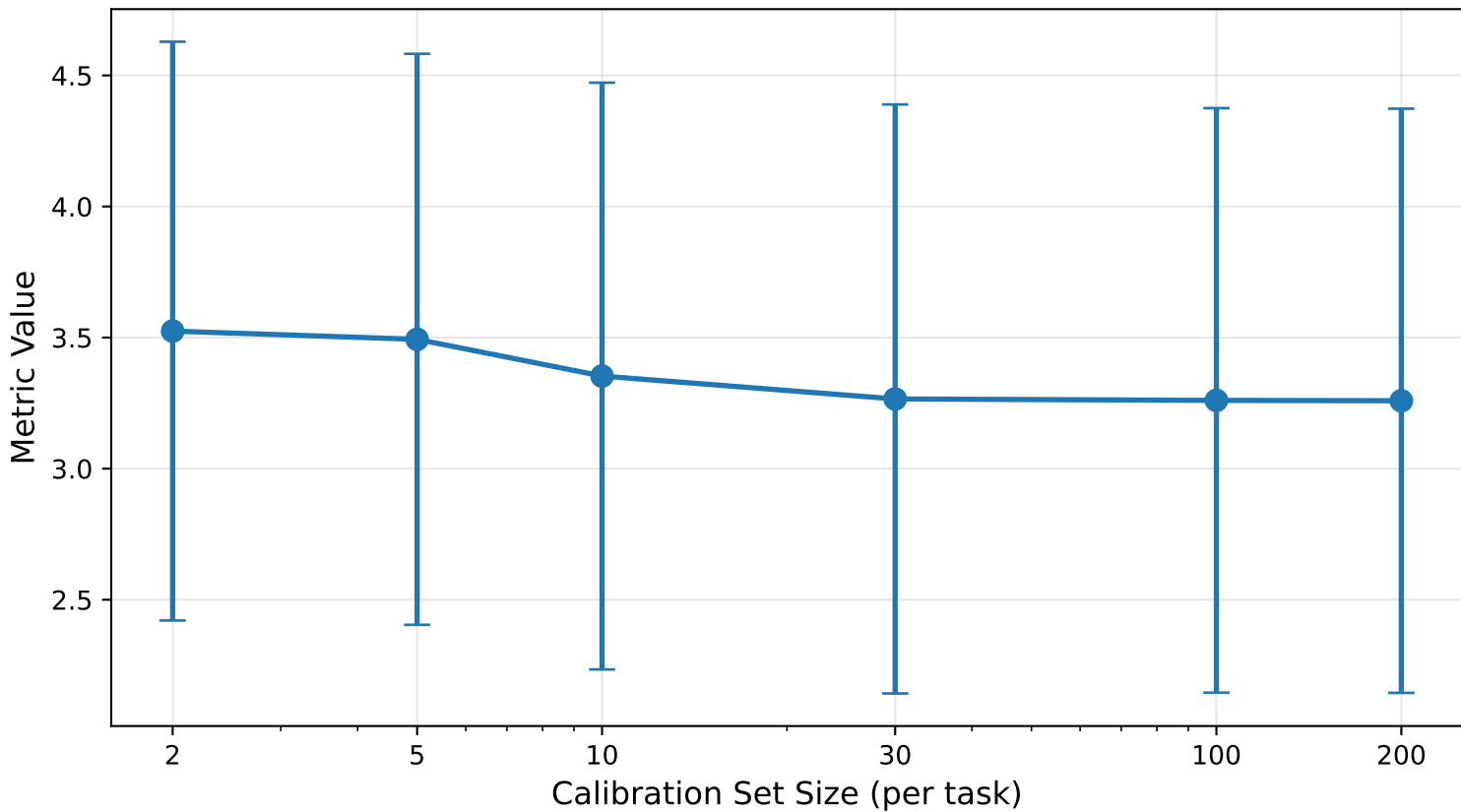
activation_l2_distance Mean \pm Std across pairs
