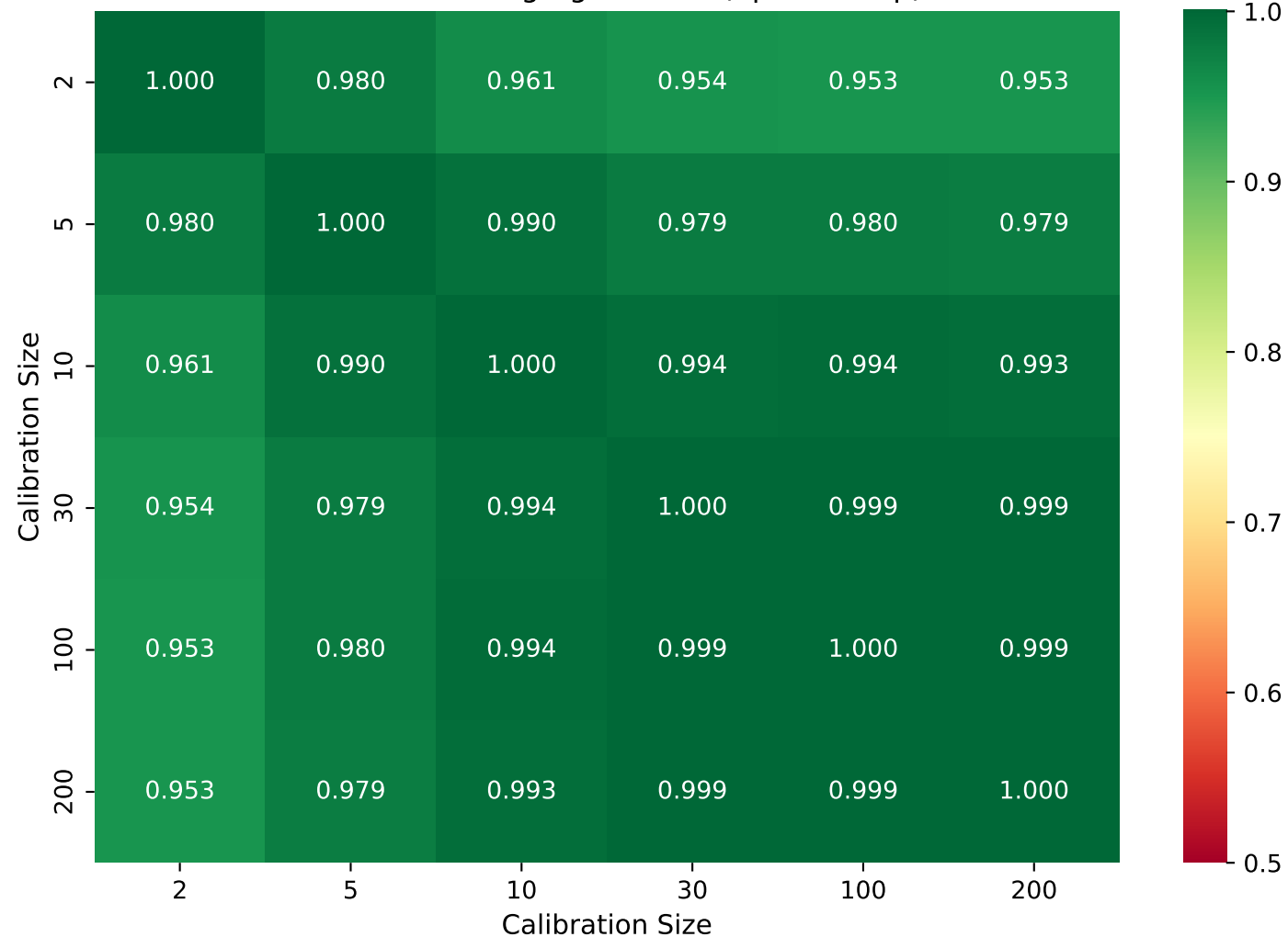
activation_dot_product Pairwise Ranking Agreement (Spearman \rho )
