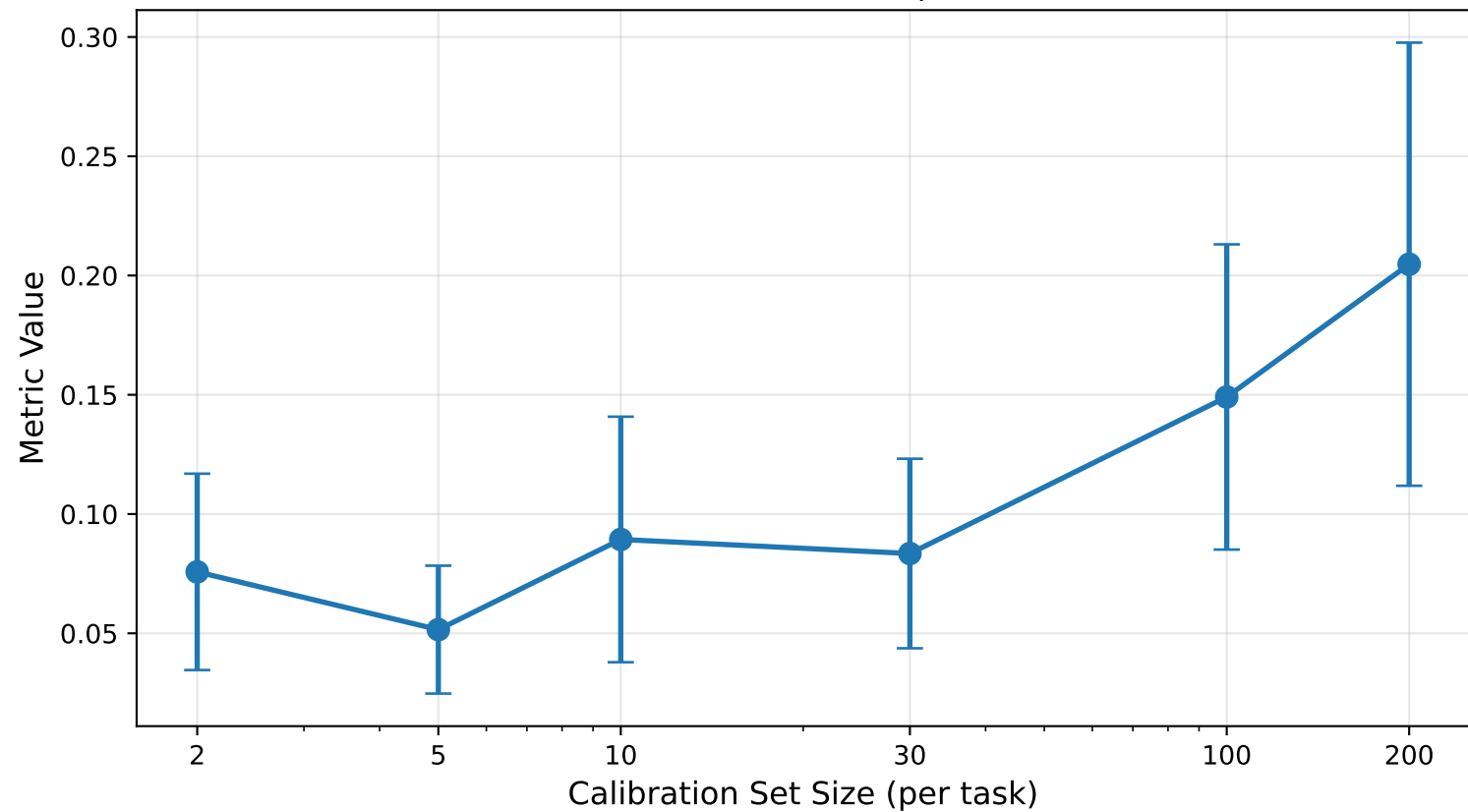
input_gradient_l2_distance Mean \pm Std across pairs
