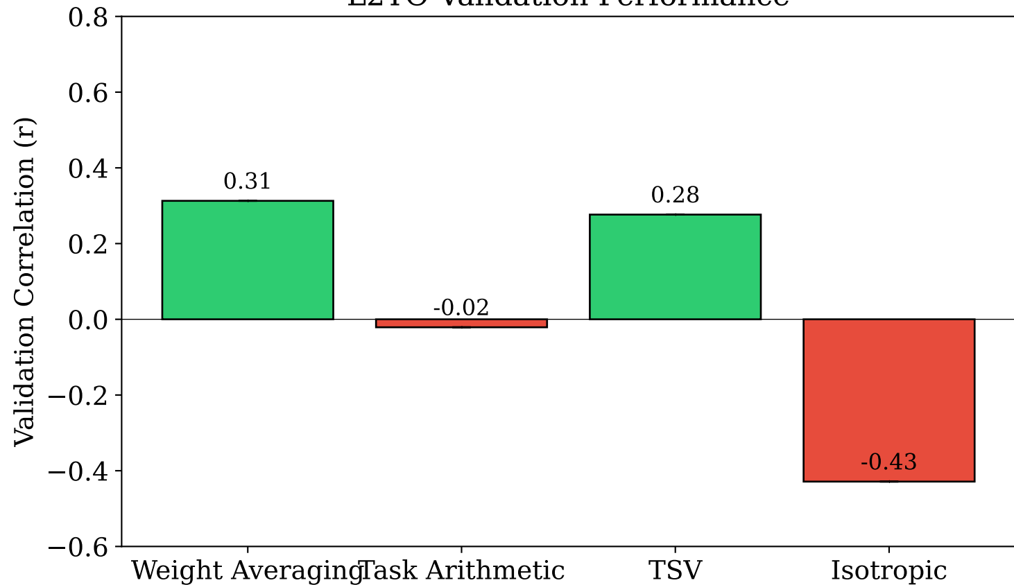
L2TO Validation Performance
