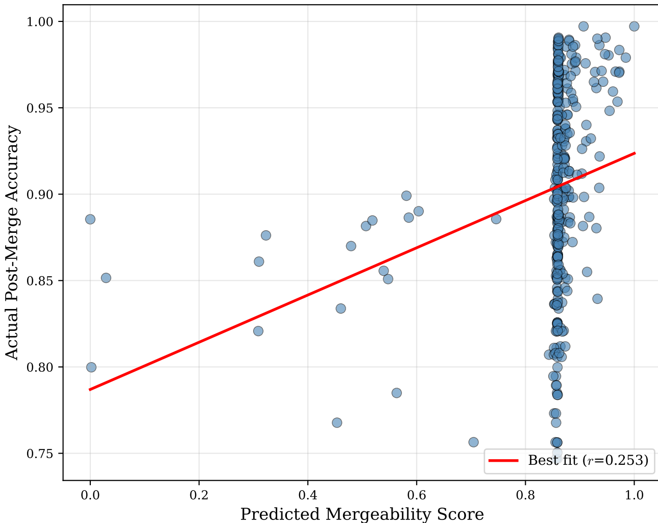
TSV: LOTO Validation Predictions ( r=0.253 , p=6.72\text{e-}07 , n=376 )
