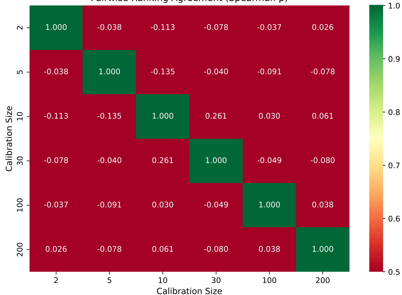
input_gradient_dot_product Pairwise Ranking Agreement (Spearman \rho )
