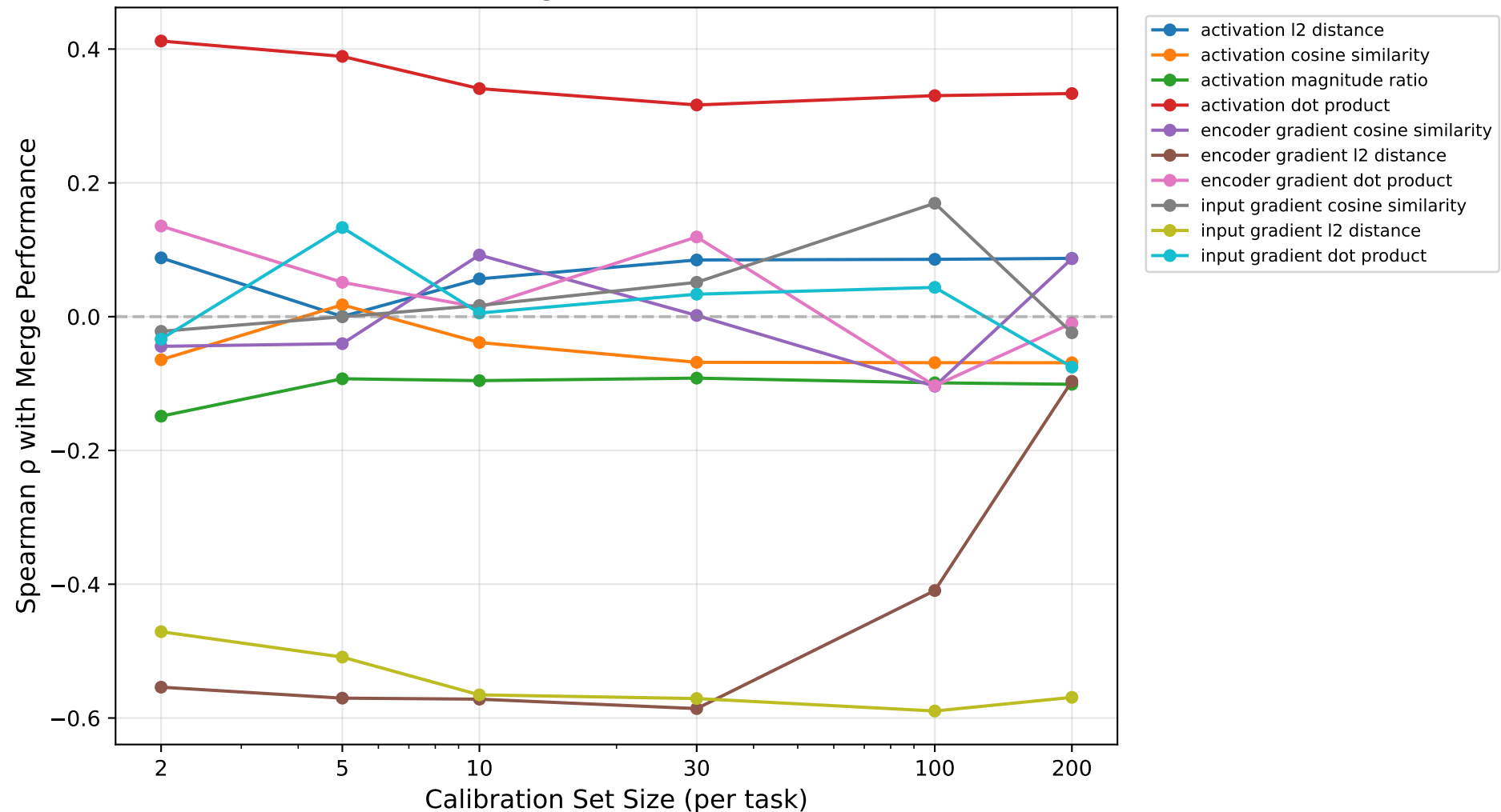
Metric-Performance Correlation vs Calibration Size (Merge Method: tsv)
