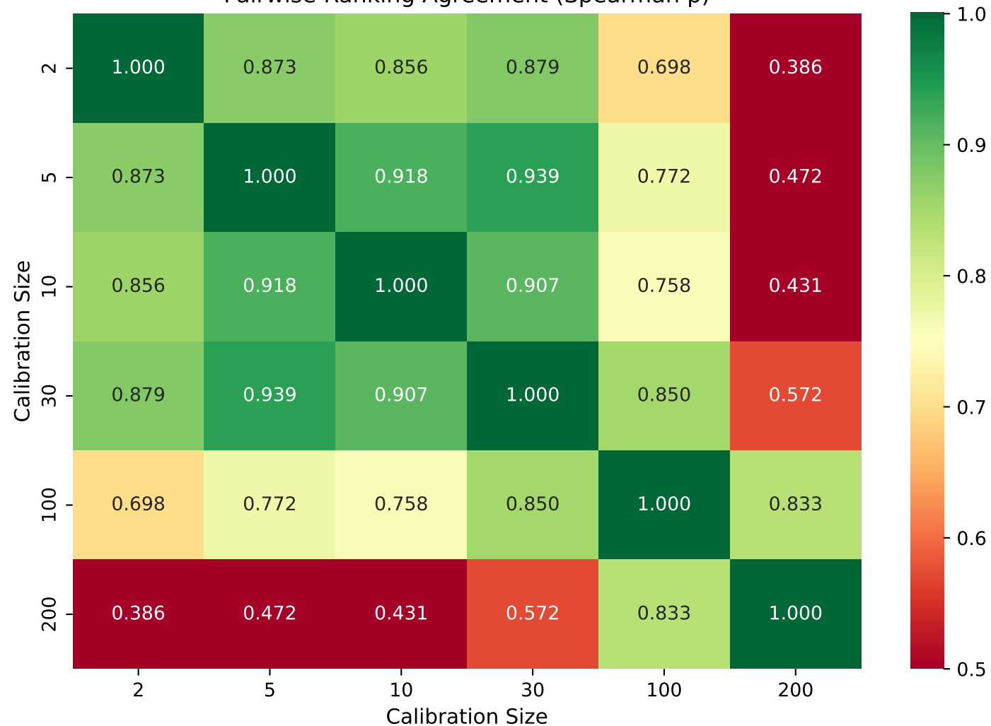
encoder_gradient_l2_distance Pairwise Ranking Agreement (Spearman \rho )
