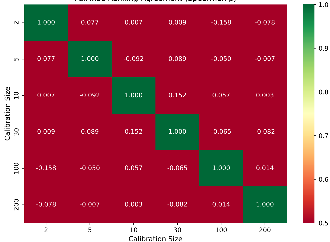
input_gradient_cosine_similarity Pairwise Ranking Agreement (Spearman \rho )
