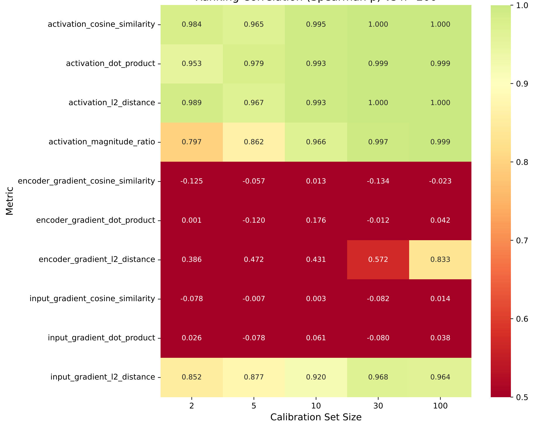
Ranking Correlation (Spearman \rho ) vs n=200
