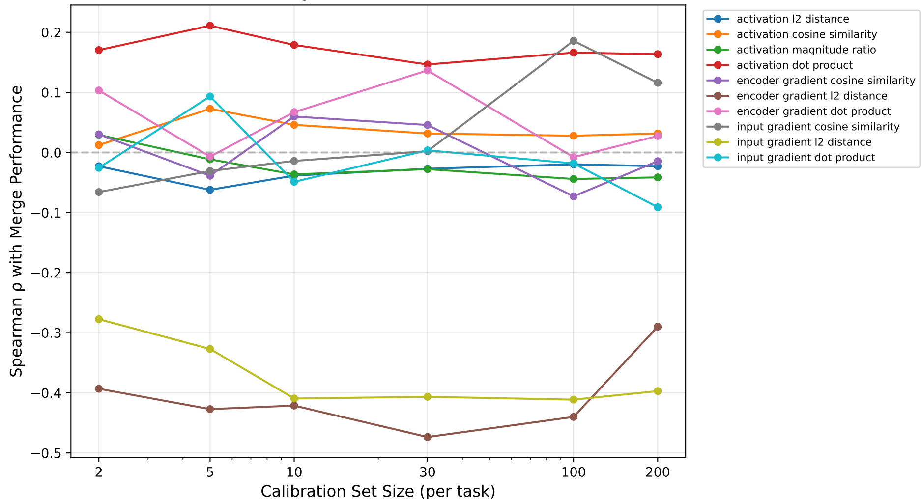
Metric-Performance Correlation vs Calibration Size (Merge Method: arithmetic)
