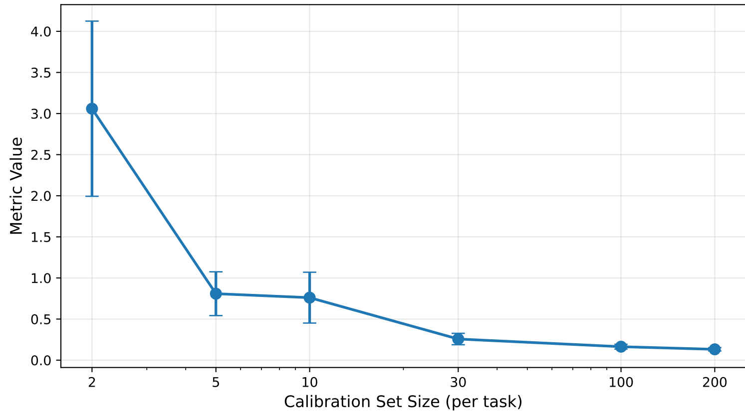
encoder_gradient_l2_distance Mean \pm Std across pairs
