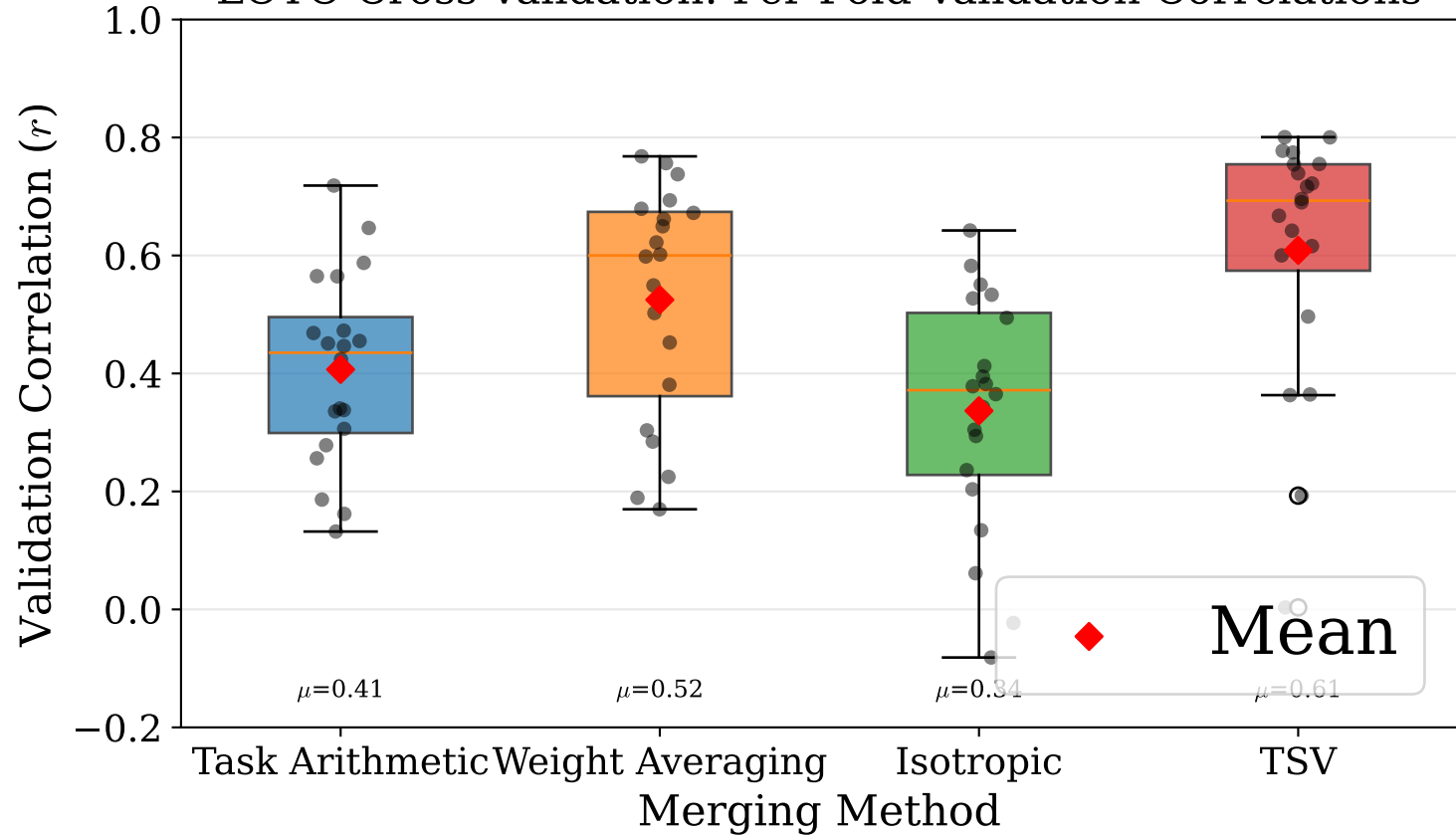
LOTO Cross-Validation: Per-Fold Validation Correlations
