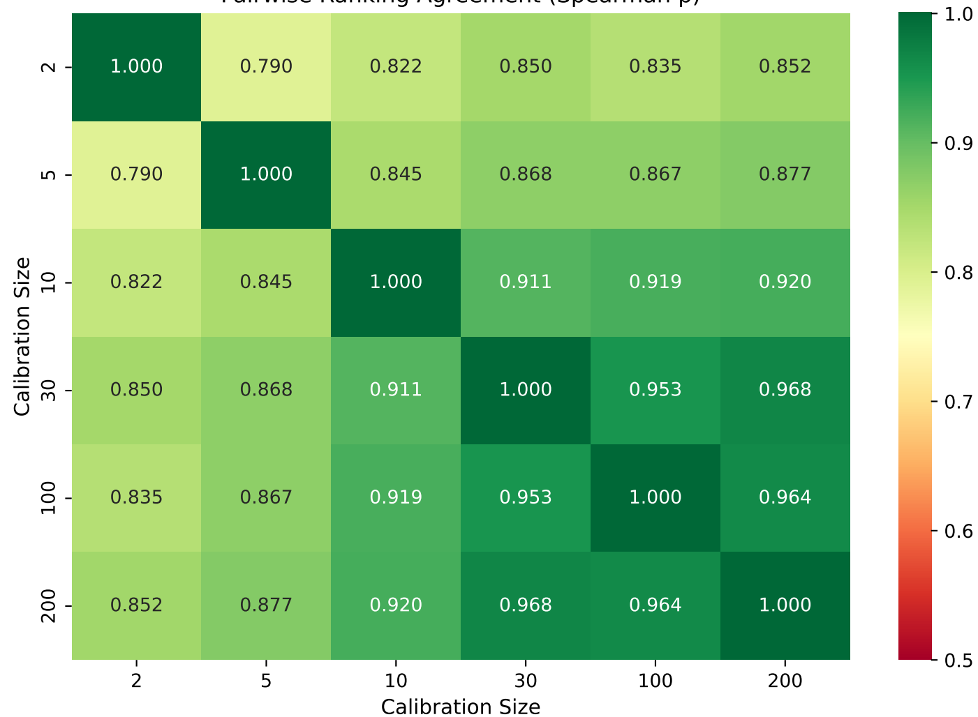
input_gradient_l2_distance Pairwise Ranking Agreement (Spearman \rho )
