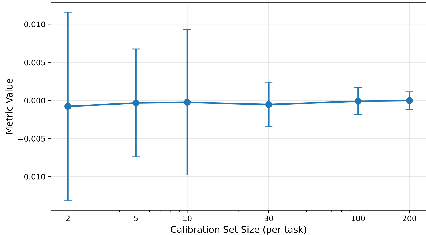
input_gradient_cosine_similarity Mean \pm Std across pairs
