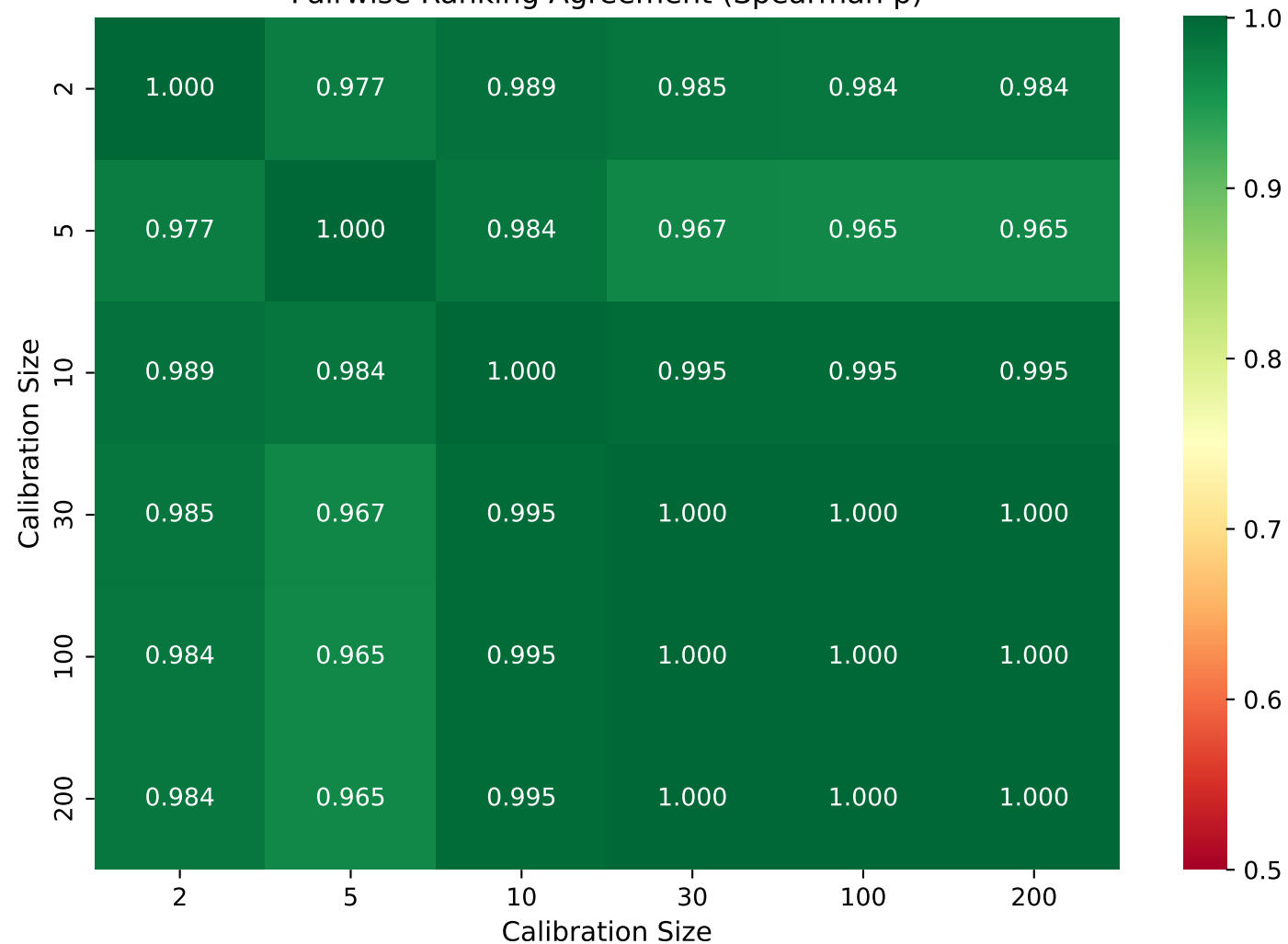
activation_cosine_similarity Pairwise Ranking Agreement (Spearman \rho )
