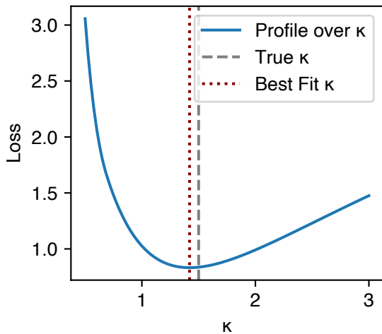
Profile Likelihood: \kappa
