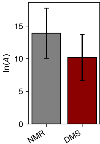
Pre-exponential Factor
