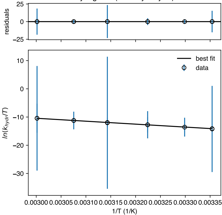
Eyring Plot (DMS hydrolysis)
