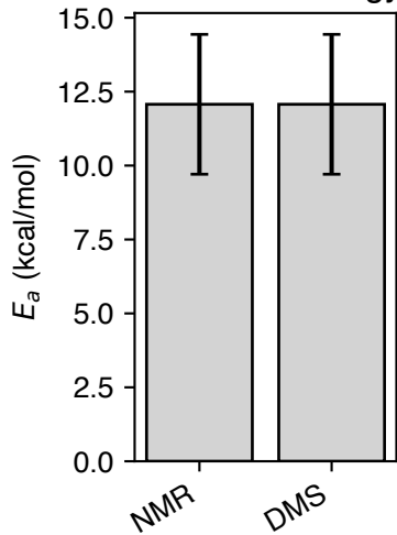
Activation Energy
