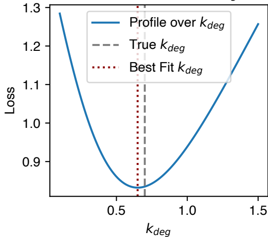
Profile Likelihood: k_{deg}
