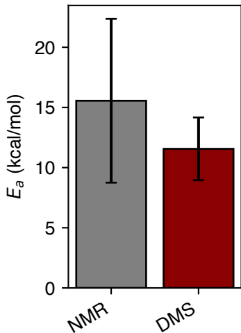
Activation Energy
