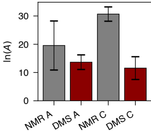
Pre-exp. Factor
