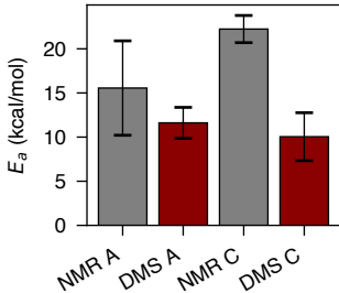
Activation Energy
